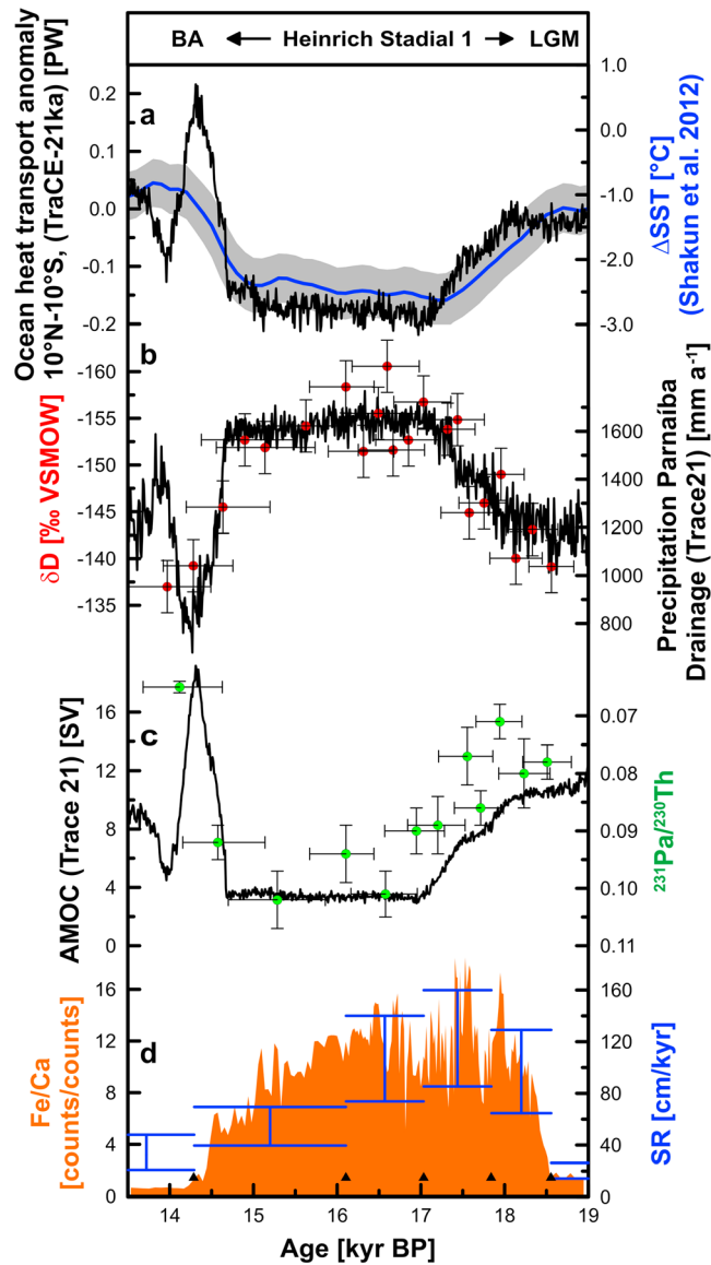
Figure 6. Modeled (TraCE-21ka [He, 2011; Liu et al., 2009]) and reconstructed evolution of AMOC, Atlantic temperature gradient, and precipitation over Heinrich stadial 1. Vertical error bars denote measurement uncertainty ( \pm 1\sigma ), horizontal error bars age uncertainty (95% range). (a) Reconstructed (blue [Shakun et al., 2012]) annual mean temperature difference between North and South Atlantic and modeled (black [He, 2011; Liu et al., 2009; Yang et al., 2015]) ocean heat transport anomaly relative to 22 thousand years B.P. (b) Ice volume corrected \delta D of n -C 29 alkane of terrestrial plant wax from core Geo16202-2 (red dots, this study) and modeled annual mean precipitation over the Parnaíba River catchment (black [Liu et al., 2009]). (c) 231 Pa/ 230 Th from core GeoB16202-2 (green circles, this study) and modeled maximum Atlantic meridional overturning (black [Liu et al., 2009]). (d) Fe to Ca ratio (red, uncalibrated counts) and 95% confidence range of mean sedimentation rate (blue, this study) between calibrated median calendar ages of radiocarbon datings (triangles, this study).
