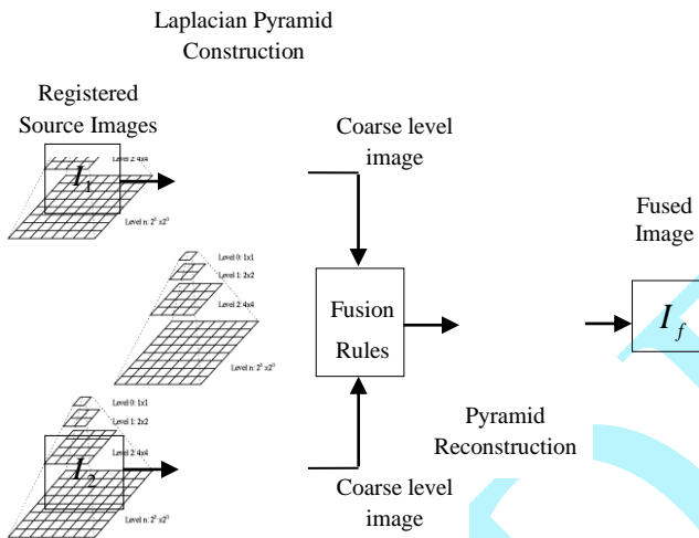
Figure 4 Laplacian Pyramid based image fusion
