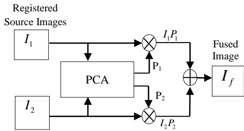
Figure 3 PCA based image fusion
