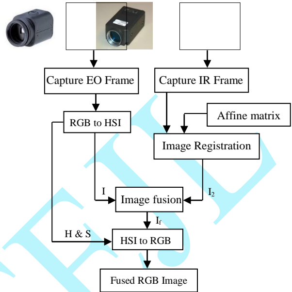
Figure 7 Steps involved in real-time image fusion
