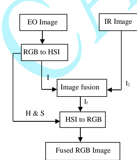
Figure 1 Steps involved in image fusion of still images
