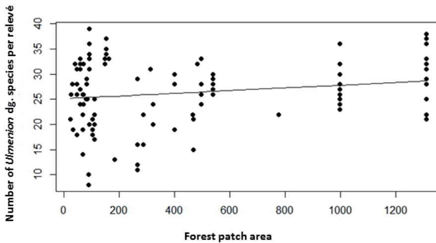
Figure 3. Relationship between number of Ulmenion diagnostic and constant species in the relevé and forest patch area (ha). The prediction line was calculated by GLM with Poisson distribution family and log-link function (with intercept 3.265, standardised estimates 0.001 and significance 0.0098).
