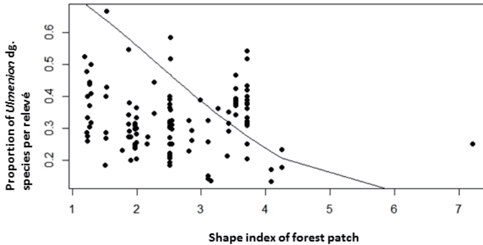
Figure 6. Relationship between the proportion of Ulmenion diagnostic species and forest patch Shape index. The prediction line was calculated by GLM with binomial distribution family weighted by species number and log-link function (with intercept 6.428, standardised estimates -7.016 and significance 0.0002).
