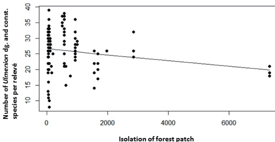
Figure 4. Relationship between number of Ulmenion diagnostic and constant species in the relevé and forest patch isolation (m). The prediction line was calculated by GLM, with Poisson distribution family and log-link function (with intercept 3.265, standardised estimates -0.001 and significance 0.0131).
