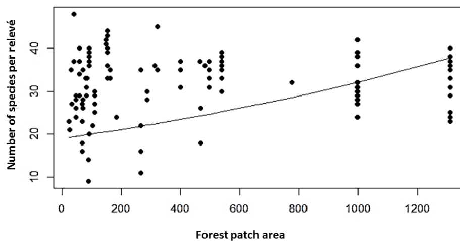
Figure 2. Relationship between the number of species in the relevé and forest patch area (ha). The prediction line was calculated by GLM with Poisson distribution family and log-link function (with intercept 2.937, standardised estimates 0.0005 and significance 0.0001).
