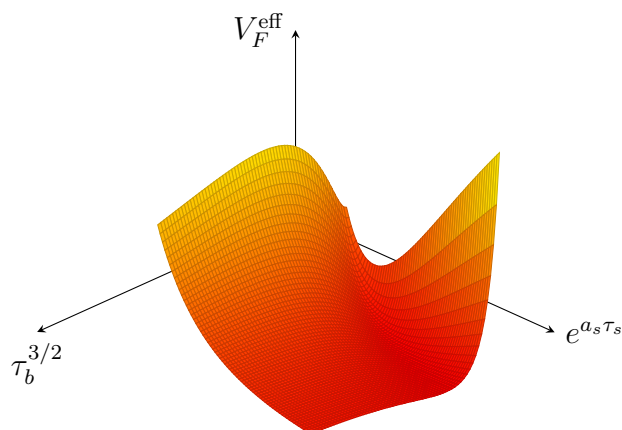
Figure 3.2. Detail of the of the scalar potential plot V_F^{\text{eff}} = V_F^{\text{eff}}(\tau_b^{3/2}, e^{a_s \tau_s}) in vicinity of the minimum: it is worthwhile to express it as a function of \tau_b^{3/2} and e^{a_s \tau_s} because in this way the two variables are roughly of the same order of magnitude in this zone. Moreover this dilatation makes it more evident the presence of a minimum.
