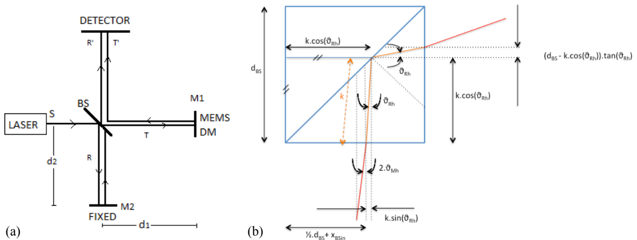
Figure 1(a): Michelson interferometer approach to demonstrate the functionality of a MEMS DM. The light from source, S, is divided by a beam splitter (BS) oriented 45 degrees to the beam. The transmitted beam travels to the MEMS deformable mirror where it is reflected back to the beam splitter. Half of the beam is deflected by 90 degrees at BS and strikes the detector. The reflected beam travels to M2 where it is reflected and half of it then passes straight through BS and reaches the detector. The two beams that are directed towards the detector interfere to produce fringes that are analytically well understood as a function of beam coherence/divergence and mirror tip/tilt 21 and that can be simulated for a variety of other different mirror shapes. Additional collimating and camera lenses not shown. 1(b): Example geometrical optics relationship of deformable mirror tip/tilt on exit angle, used in an ongoing study to optimize the component placement and mirror stroke selection.
