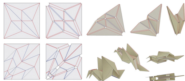
Fig. 9 Numerical folding simulation of two thickened crease patterns using Freeform Origami
