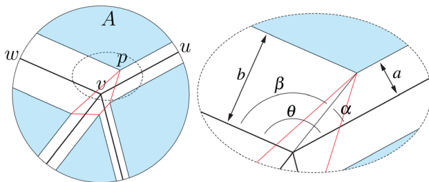
Fig. 3 Polygon construction. A generic internal crease-pattern vertex showing relationship between offsets and angles.
