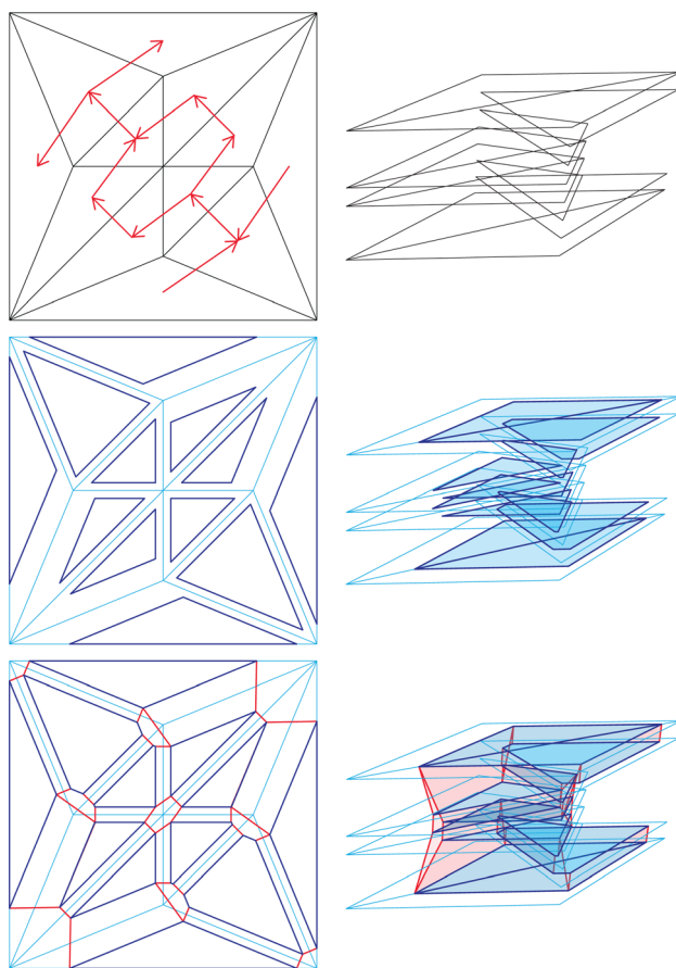
Fig. 8 Construction process
