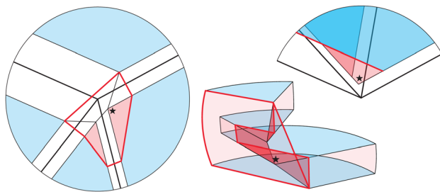
Fig. 5 Trimming intersecting region
