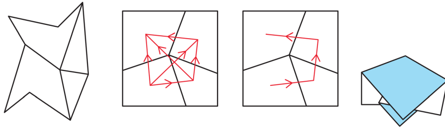
Fig. 2 From left to right: (1) generic crease pattern \Xi_0 , (2) locally flat-foldable crease pattern \Xi with layer ordering graph \Lambda , (3) with reduced layer ordering graph \Gamma , and (4) flat folding f_{\Xi}(\Xi)
