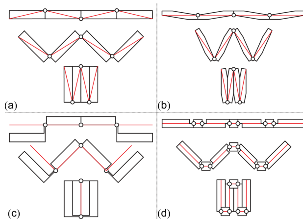
Fig. 1 Some existing thick folding techniques: (a) hinge shift, (b) volume trimming, (c) offset panel, and (d) offset crease
