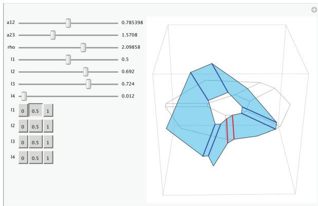
Fig. 10 Parameterized thick single-vertex construction in Mathematica
