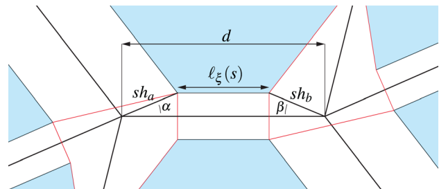
Fig. 7 Scale factor calculation showing relevant quantities
