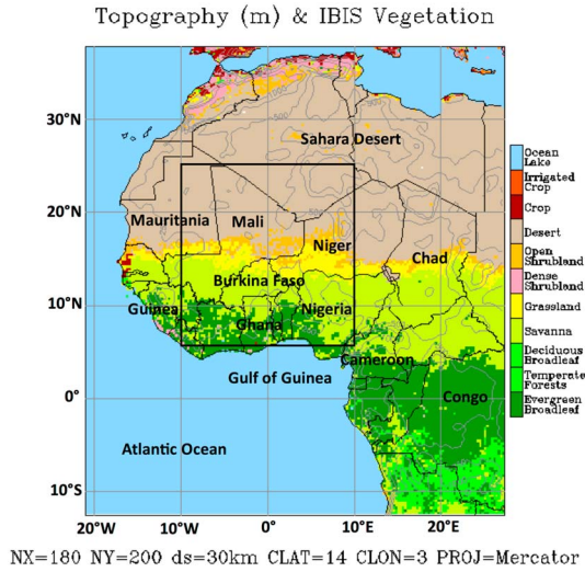
Figure 1. Domain implemented for RegCM3-IBIS simulations. Vegetation biomes are shaded and topography (in meters) contoured. Boxed region shows area where spatial averages are computed for ( 10^{\circ}\text{W} – 10^{\circ}\text{E} , 6^{\circ}\text{N} – 25^{\circ}\text{N} ).
