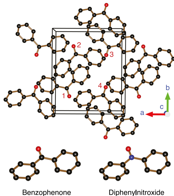
FIG. 1. (Top) Crystal structure of benzophenone. The crystal has space group symmetry P2_12_12_1 with four molecules per unit cell. Molecules 1–4 are of the same unit cell represented by the rectangular parallelepiped. Molecules 2–4 are 180^\circ rotated about the crystallographic a , b , and c axes, respectively, with respect to molecule 1. (Bottom) Molecular structures of benzophenone (left) and diphenylnitroxide (right) with oxygen atoms in red, nitrogen in blue, and carbon atoms in black. The figure was rendered in VESTA software. 44
