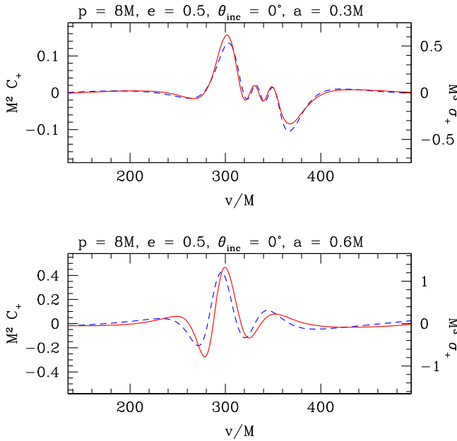
FIG. 8. Applied tidal field vs shear response for eccentric equatorial orbits of spinning black holes. Data in both panels are for an orbit with p = 8M , e = 0.5 , \theta_{\text{inc}} = 0^\circ , and include modes up to l = 9 . The top is for a hole with spin a = 0.3M , and the bottom is for a hole with spin a = 0.6M . As in Fig. 7, we show the on-horizon Weyl curvature polarization C_+ [dashed (blue) curve] and the shear polarization \sigma_+ that results [solid (red) curve]. All data are plotted at \theta = 90^\circ , \psi = 0^\circ .
