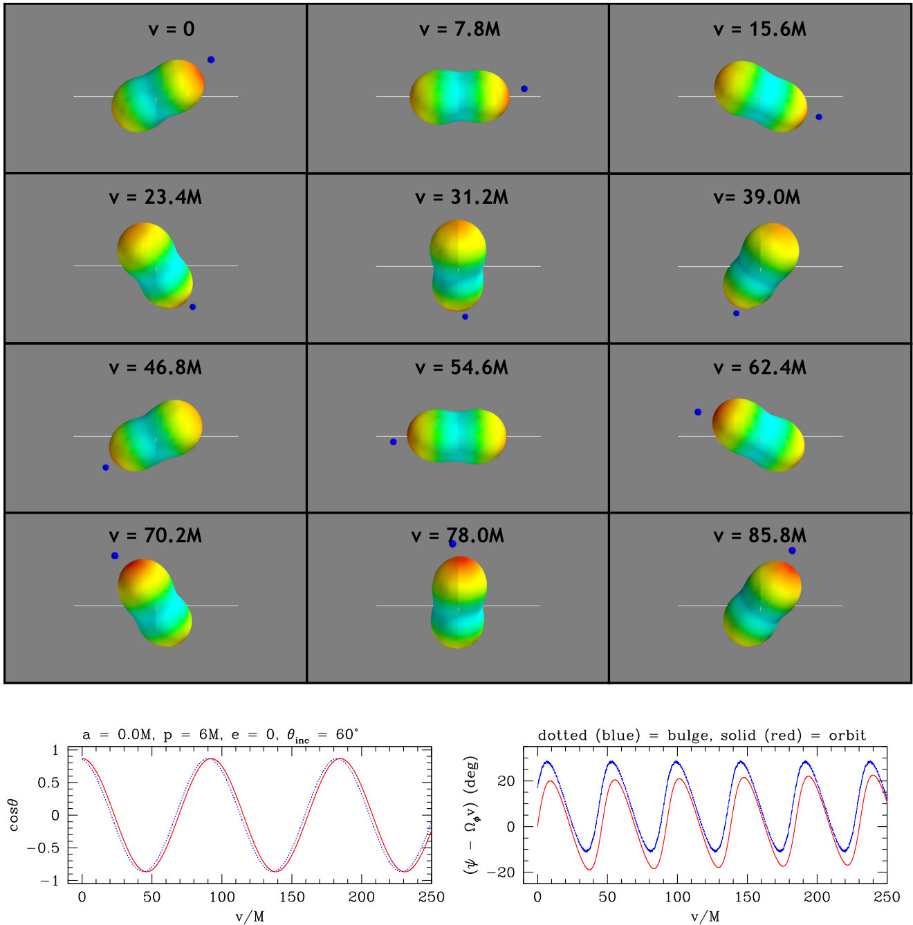
FIG. 12. Top: Snapshots of an animation depicting an embedding of the distorted horizon for a circular inclined orbit of a Schwarzschild black hole ( a = 0 ). Bottom: Angular position of the horizon’s bulge [dotted (blue) curve] vs the angular position of the orbiting body [solid (red) curve]. The orbit is at radius r = 6M , inclined at \theta_{\text{inc}} = 60^\circ to our chosen equatorial plane. The axes shown in these snapshots indicate the hole’s equatorial plane; we have placed the camera slightly above this plane in order to illustrate the hole’s bulge geometry. The orbiting body is indicated by the small moon (dark blue in the color plot) located near one of the horizon bulges. The small body’s orbit begins on the side of the black hole near the camera, descends down through the equatorial plane (crossing just after v = 7.8M ), sweeps behind the far side of the hole (moving from right to left as plotted), then comes up through the equatorial plane (crossing just after v = 54.6M ) to pass in front of the side near the camera again. The animation from which these stills are taken is available in Ref. [28]. The bottom two panels show the angular position of the bulge and the orbit, illustrating the polar angle ( \cos \theta , left) and the axial angle ( \psi , right). The horizon’s bulge moves in lockstep with the orbiting body, always leading the orbit by a small, constant angle.
