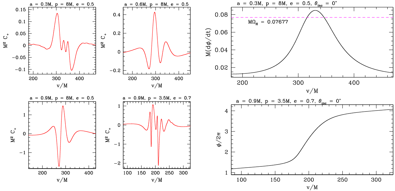
FIG. 4. Examples of the on-horizon tidal field C_+ for equatorial eccentric orbits of Kerr black holes (left) and features of the orbits which we use to explain some of the behavior we find (right). The cases shown here demonstrate several examples of interesting behavior for strong-field Kerr orbits. On the left, the top panels and the bottom left panel are for orbits with p = 8M, e = 0.5 and show orbits about black holes with spins a = 0.3M, a = 0.6M , and a = 0.9M ; the bottom right panel on the left is for an orbit with p = 3.5M, e = 0.7 about a black hole with a = 0.9M . In all cases, we examine the field at \theta = 90^\circ, \psi = 0^\circ ; C_+ vanishes there for all equatorial orbits. The behavior we see in the top right and bottom left panels is very similar to the prototype behavior of C_+ we saw in Fig. 3: a large spike coinciding with periapse passage and smaller-scale oscillations before and after. The behavior we see in the top left and bottom right deviates from the prototype in interesting ways. For a = 0.3M, p = 8M, e = 0.5 , C_+ undergoes additional very small-amplitude oscillations during the spike. On the right, the top panel compares the orbit’s axial speed d\phi/dt with the horizon’s spin frequency \Omega_H . The small-amplitude oscillations occur during the brief span in which d\phi/dt exceeds \Omega_H . For a = 0.9M , there are multiple high-amplitude oscillations near the largest spike. This is correlated with “whirling” orbital dynamics. As shown in the bottom panel on the right, the orbit wraps around the black hole multiple times at periapsis before “zooming” back out to apoapsis.
