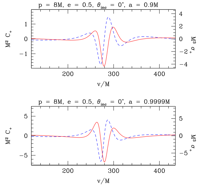
FIG. 9. Applied tidal field vs shear response for eccentric equatorial orbits of spinning black holes. Data in both panels are for an orbit with p = 8M , e = 0.5 , \theta_{\text{inc}} = 0^\circ , and include modes up to l = 9 . The top is for a hole with spin a = 0.9M , and the bottom is for a hole with spin a = 0.9999M . As in Figs. 7 and 8, we show the on-horizon Weyl curvature polarization C_+ [dashed (blue) curves] and the shear polarization \sigma_+ that results [solid (red) curves]. All data are plotted at \theta = 90^\circ , \psi = 0^\circ .
