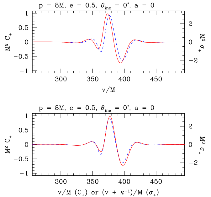
FIG. 7. Applied tidal field vs shear response for an eccentric equatorial orbit of a nonspinning black hole. Data are for an orbit with p = 8M , e = 0.5 , \theta_{\text{inc}} = 0^\circ . We show the on-horizon Weyl curvature polarization C_+ [dashed (blue) curves] as well as the resulting shear polarization \sigma_+ [solid (red) curves]. Both fields are plotted at \theta = 90^\circ , \psi = 0^\circ and include all modes up to l = 9 . The top panel shows C_+ and \sigma_+ as functions of ingoing time v . Notice that \sigma_+ appears to lead C_+ by an almost constant time interval. The bottom panel shows the same data, but with \sigma_+ shifted by \Delta v = \kappa^{-1} = 4M . The shear response lines up almost perfectly with the driving tide in this panel, showing that the shear \sigma_+ leads the tide by \kappa^{-1} in the Schwarzschild limit.
