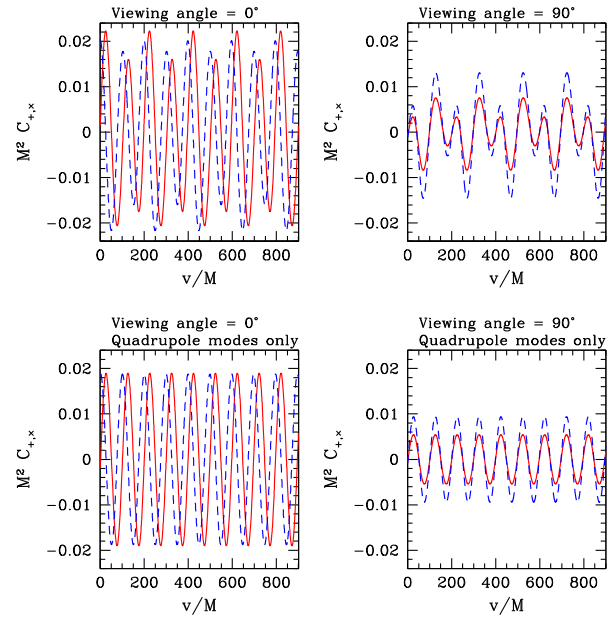
FIG. 1. Examples of the on-horizon tidal field C for circular orbits around a Schwarzschild black hole. The four plots shown here are for an orbit with p = 10M and with inclination angle \theta_{\text{inc}} = 60^\circ . The solid (red) line shows the polarization C_+ ; the dashed (blue) line shows C_x . The top two panels illustrate how this field varies with ingoing time v at azimuth angle \psi = 0^\circ and \psi = 90^\circ ; the bottom two figures show the same data, but including only quadrupolar modes (i.e., modes for which l=2 and m+k = \pm 2 ). These plots illustrate the importance of modes beyond the quadrupole, as well as the strong functional dependence of the tide on the position at which it is measured.
