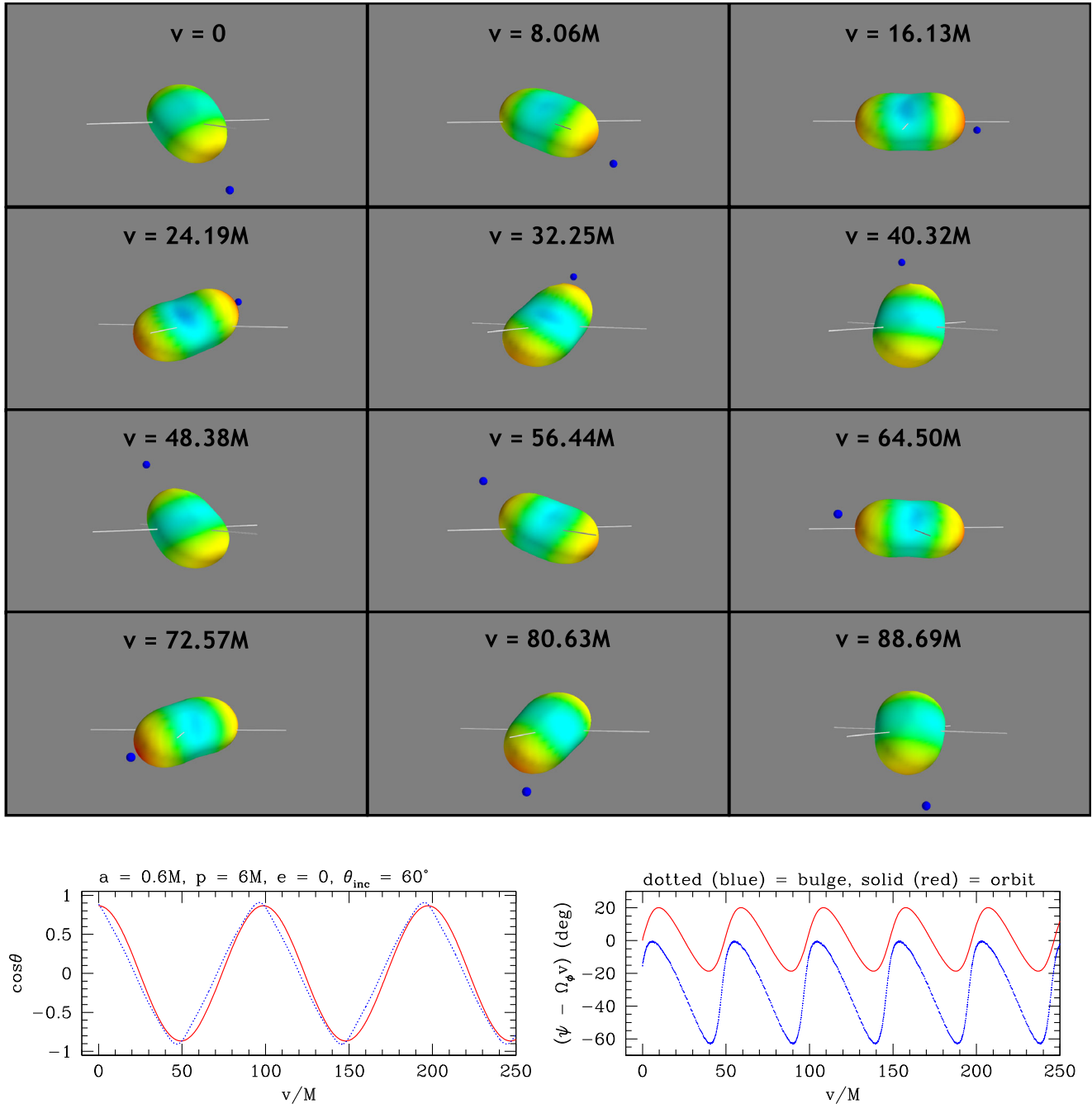
FIG. 13. Identical to Fig. 12, except that the black hole shown here is spinning with Kerr parameter a = 0.6M . As in Fig. 12, the axes indicate the hole’s equatorial plane. In this plot, these axes rotate with the event horizon at frequency \Omega_H = a/2Mr_+ = 1/6M (corresponding to a rotation period T_H = 2\pi/\Omega_H = 37.7M ). In this sequence, the orbiting body (small sphere, dark blue in color) begins near the face close to the camera on the lower right-hand side of the black hole. It then sweeps up, crossing the equator soon after v = 16.13M ; passes behind the black hole; and then descends downward again, crossing the equator soon after v = 64.5M . The horizon’s distortions in this case do not move in lockstep with the orbiting body. Instead, the horizon exhibits mild shape variations. This is because the hole is not spherically symmetric, and so the tidal field acting on the horizon varies slightly over the orbit. Notice that the horizon’s bulge leads the angular position of the orbit in the polar ( \theta ) direction but lags its position in the axial ( \psi ) direction; this can be seen in the snapshots but is especially clear in the angle vs time plots shown in the bottom two panels. (We subtract \Omega_\phi v from \psi to remove the uninteresting secular growth in this angle over a single orbit.) The polar behavior is much like what we see for Schwarzschild or very slow rotation; the axial behavior is about the same as the behavior we saw for equatorial circular orbits in paper I. The animation from which these stills are taken is available in Ref. [28].
