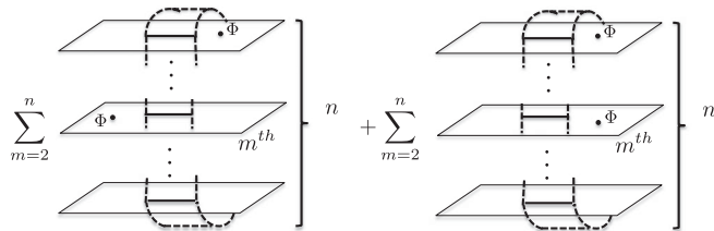
FIG. 3. The type of two-point functions on the replica manifold whose analytic continuation determines quantum Fisher information in vacuum.
