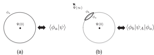
FIG. 1. (a) Operator-state correspondence in radial quantization of conformal field theories. (b) Reduced density matrix corresponds to a path integral with two operator insertions and a cut on the subsystem.
