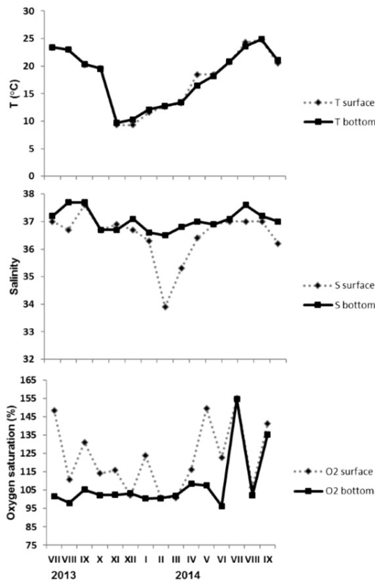
Fig. 6. Oxygen saturation (%), temperature ( ^{\circ}\text{C} ) and salinity for surface and bottom layers at investigated sites
