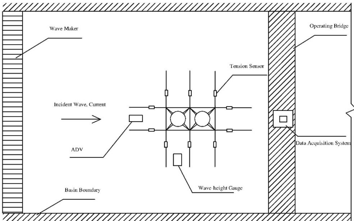
Figure 2. Test model arrangement.
