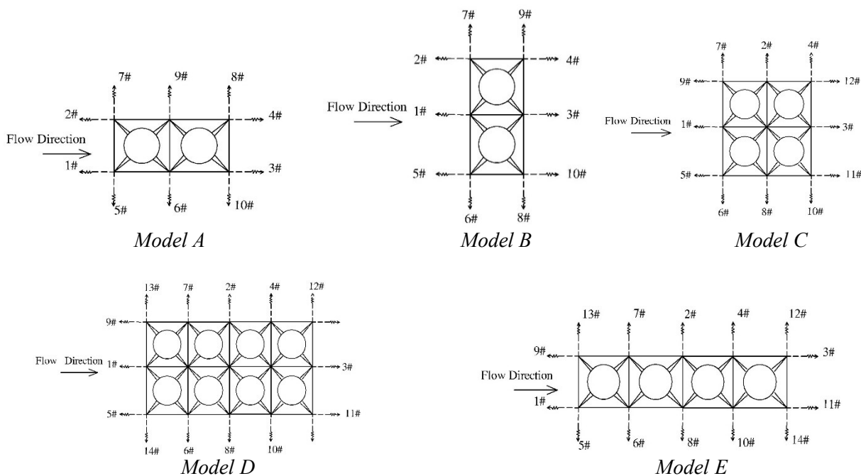
Figure 1. Composite-type sea cage combined mode.
