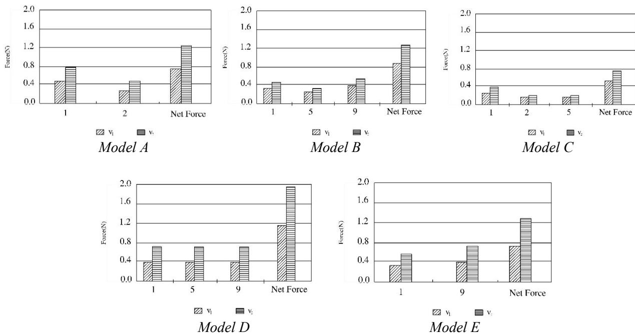
Figure 3. The forces exhibiting on current model.
