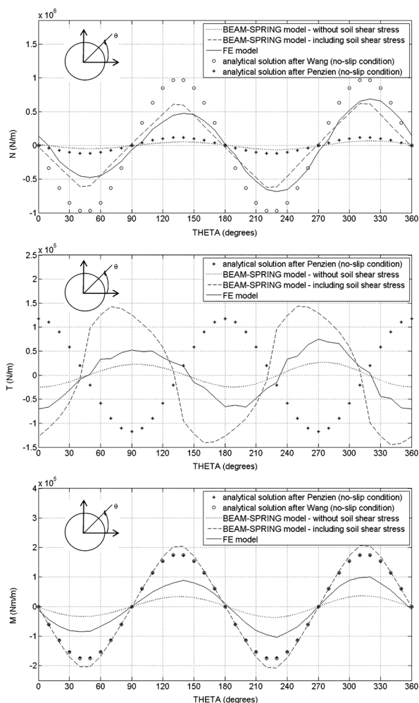
Figure 7 Comparison of numerical dynamic analysis results with analytical solutions after Wang, 1993 [10] and Penzien, 2000 [12]
