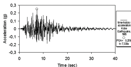
Figure 4 Acceleration record used in 1D SSR analysis
