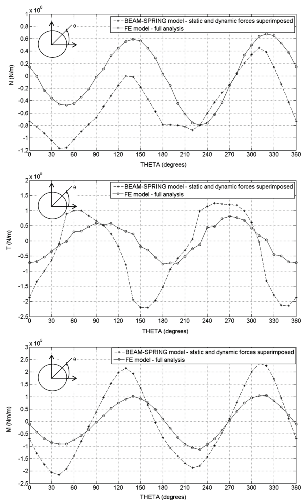
Figure 10 Comparison of the models regarding the lining force distributions under total loading
