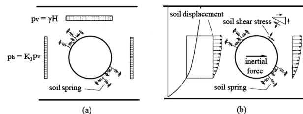
Figure 2 Discrete beam-spring model: (a) static analysis; (b) dynamic analysis
