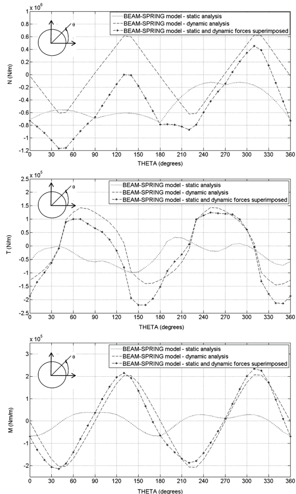
Figure 8 Numerical results of the lining force distributions under static, dynamic, and superimposed effects using the beam-spring model
