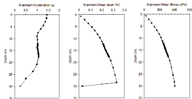
Figure 5 Maximum acceleration, shear strain, and shear stress profiles obtained by the 1D SSR linear analyses
