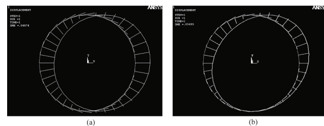
Figure 6 Different ovaling deformation shapes of the circular tunnel cross-section: (a) beam-spring model without soil shear stress; (b) beam-spring model accounting for soil shear stress
