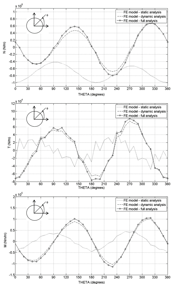
Figure 9 Numerical results of the lining force distributions under static, dynamic, and total loading conditions using the continuous FE model
