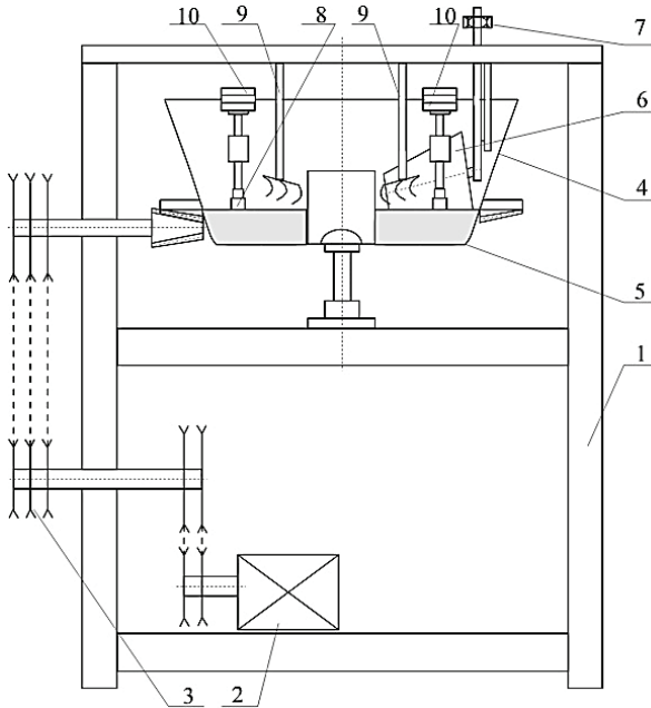
Figure 1 A stand for examination of wear in abrasive soil pulp: 1 - frame, 2 - motor, 3 - belt transmission, 4 - bowl, 5 - soil, 6 - pressing rollers, 7 - roller pressing, 8 - grip with sample, 9- scarfing fork, 10- sample weights
