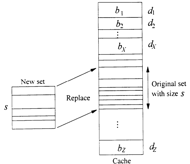
Fig. 1. Cache Optimality.
