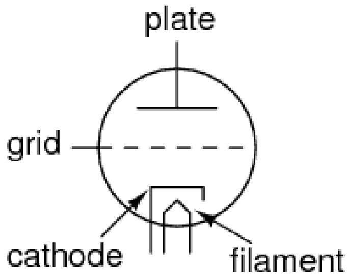
Figure 3.2.1: Triode Diagram
