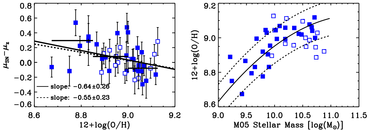
Figure 12. Left-hand panel: relationship between gas-phase metallicity and HR for purely star-forming galaxies (blue solid points) and transition galaxies (open blue points). The solid line and the dashed line denote least-squares fits to all data points and to solid data points, respectively. The slopes and corresponding errors are given by the labels. The horizontal lines denote median HR in bins of the x -axis parameters with lengths according to the width of the bins for all data points. Right-hand panel: relationship between gas-phase metallicity and stellar mass; the same symbols as in the left-hand panel. The solid curve shows the relation from Tremonti et al. (2004) with 1\sigma errors (dashed curves).
