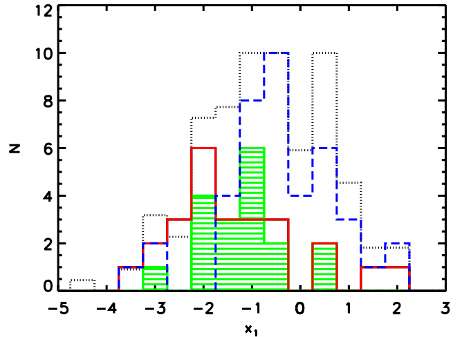
Figure 7. Distribution of the stretch factor x_1 for the different emission classifications (see Section 3.1). The blue (dashed open) histogram represents star-forming, the green (filled) represents AGN and the red (solid open) represents passively evolving galaxies. The dotted histogram shows a sample of objects with z < 0.21 , but without the separation and host spectroscopy cuts applied, normalized to peak at N = 10 .
