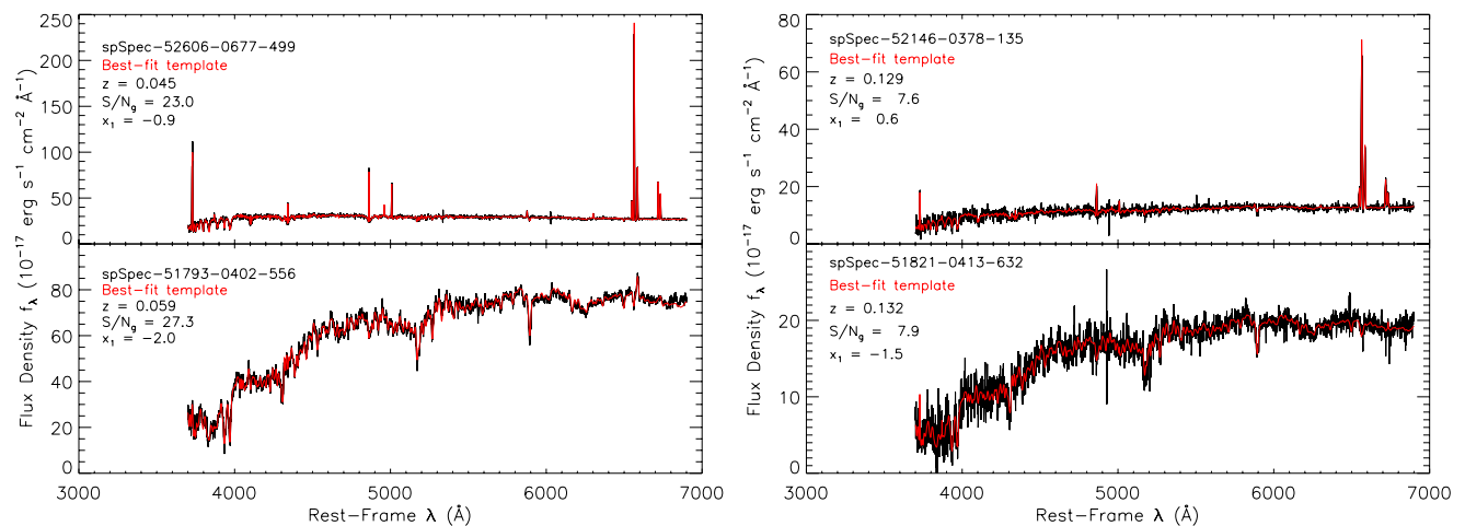
Figure 1. Four examples of host galaxy spectra (black SEDs) at rest-frame wavelength and with the best-fitting model templates from GANDALF/PPXF (red SEDs) overlaid. The top and lower panels show galaxies hosting SNe Ia with large and small stretch factor values, respectively, as given by the labels. The left- and right-hand panels show high- and low-S/N spectra, with values given by the labels. The redshift for each object is also indicated by the labels.
