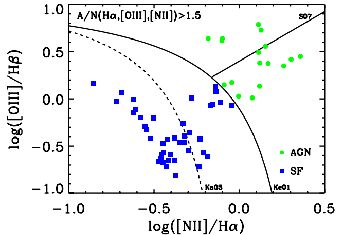
Figure 4. BPT diagram for the 59 galaxies with detected emission lines, i.e. AoN > 1.5 for \text{H}\alpha , [\text{O III}](\lambda 5007) and [\text{N II}](\lambda 6584) . The blue squares denote star-forming galaxies and the green circles exhibit AGN activity only. The solid curved line shows the theoretical star formation limit from Kewley et al. (2001, Ke01) and the dashed curved line shows the empirical separation of AGN and purely star-forming galaxies from Kauffmann et al. (2003b, Ka03). Objects that fall between these lines are transition objects, hosting both star formation and AGN activity. The separation of LINERs and Seyfert AGNs from Schawinski et al. (2007, S07) is indicated by the solid straight line.
