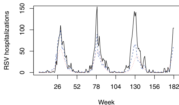
Figure 10: Real hospitalizations for RSV (solid line) and simulated numbers of hospitalizations provided by both the Bayesian stochastic SIRS model (dashed line) and the deterministic continuous-time model (dotted line) for a coverage rate \nu = 0.2 .
