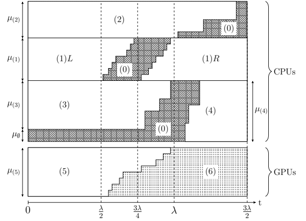
Fig. 1: Structure of the schedule. The number of processors used by set (i) is denoted by \mu(i) . The number of CPUs below set (3) is denoted by \mu_0 .
