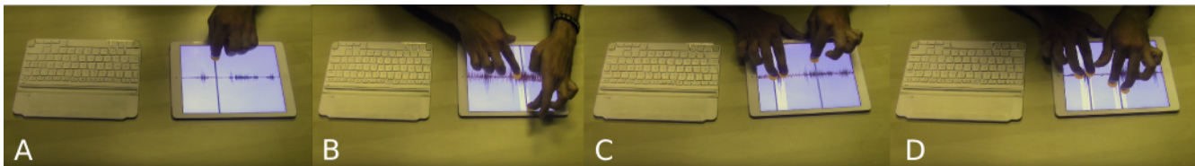
Figure 3: The advanced functionalities introduced by the VRM represented in terms of its incremental touch interaction: (A) one finger in the tablet screen results in control of the playback position; (B) two fingers result in redefining the looping area; (C) three fingers result in controlling the playback position and redefining the looping area; and (D) four fingers result in two looping areas playing in parallel.
