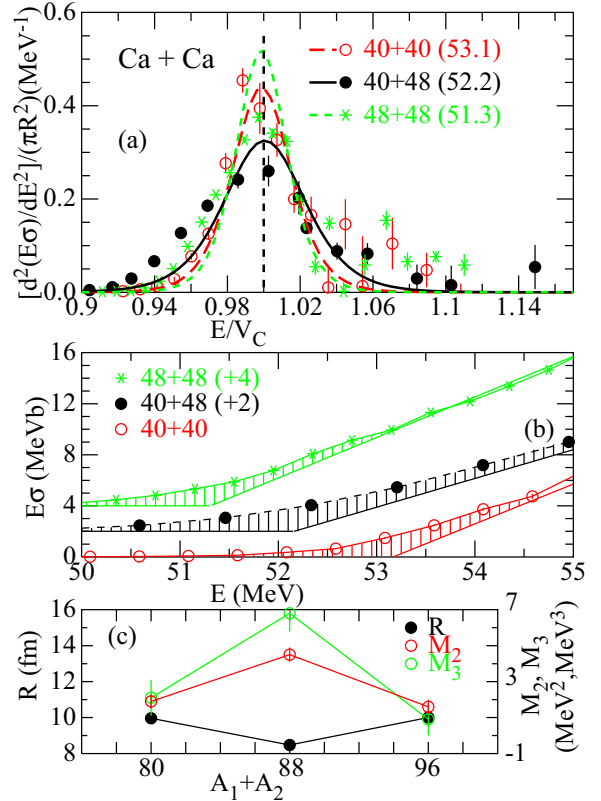
FIG. 6. (a) Barrier distributions for three Ca + Ca fusion reactions. The ^{40}\text{Ca} + ^{48}\text{Ca} system (black) exhibits the widest distribution (large M_2 ) and the lowest maximum (small R ). The symbols are obtained from calculating the second derivative of the energy-weighted, high-statistics cross sections. The curves are the barrier distributions B_w(E) of the Wong model [Eq. (11)]. (b) Plot of E\sigma vs E for energies close to the barrier. The second moment M_2 is calculated from the cross-hatched area, which is largest for the ^{40}\text{Ca} + ^{48}\text{Ca} system shown in black. (c) Plot of R , M_2 , and M_3 vs A_1 + A_2 .
