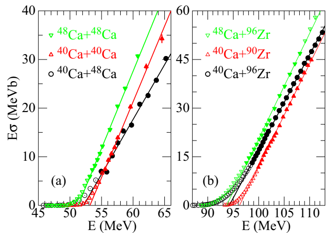
FIG. 2. Plots of E\sigma vs E for the fusion systems Ca + Ca and Ca + Zr. The straight lines are least-squares fits of Eq. (4) to the data at high energies (solid circles). The slopes of these lines determine the \pi R^2 values for each system.
