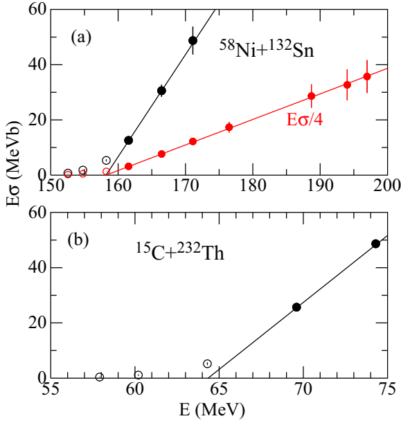
FIG. 5. Plots of E\sigma vs E for two systems with radioactive beams, (a) ^{58}\text{Ni} + ^{132}\text{Sn} and (b) ^{15}\text{C} + ^{232}\text{Th} . The red line and symbols in panel (a) show the data plotted on a reduced scale. The solid circles are data used in the least-squares fits using Eq. (4).
