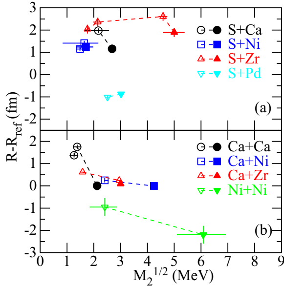
FIG. 3. Plots of R - R_{\text{ref}} vs \sqrt{M_2} for S-induced (a) and Ca- and Ni-induced (b) fusion reactions listed in Table II (the results for O, Si + Sm, and O + W are not included). Systems with the same Z_1 and Z_2 are connected by dashed lines. Systems that exhibit strong transfer reactions are shown by solid points (see text for details).
