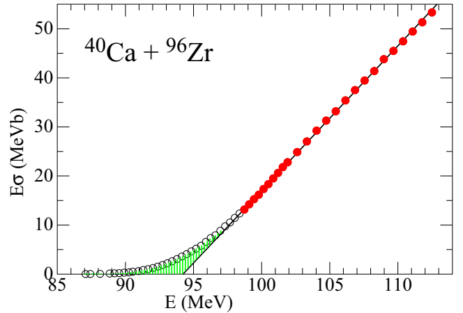
FIG. 1. Plot of E\sigma vs E for the fusion reaction ^{40}\text{Ca} + ^{96}\text{Zr} . The black line is given by the equation \pi R^2(E - V_C) with the parameters R and V_C obtained from a least-squares fit to the data at E > 1.04V_C (red solid circles). The second and third moments M_2 and M_3 are calculated from the green-shaded area. See text for details.
