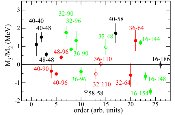
FIG. 4. Plot of M_3/M_2 , for systems where the uncertainties allow the calculation of a meaningful value of (M_3/M_2) . The x axis is the order in which the systems are quoted in Table II.
