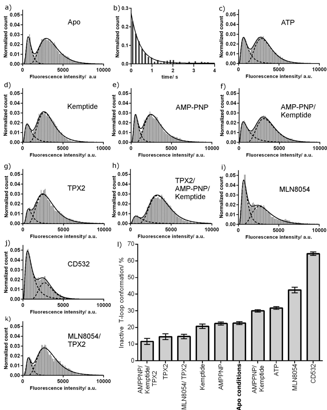
Figure 2. Fluorescence intensity distribution for phosphorylated TMR-labeled K224C/S283C Aurora A. a) Intensity histogram of unliganded Aurora A. b) Dwell time histogram of the quenched inactive T-loop conformation. c–k) Fluorescence intensity distributions with c) 1 mM ATP, d) 3 mM kemptide, e) 1 mM AMP-PNP, f) 1 mM AMP-PNP and 3 mM kemptide, g) 5 \mu M TPX2, h) 5 \mu M TPX2, 1 mM AMP-PNP, and 3 mM kemptide, i) 10 \mu M MLN8054, j) 10 \mu M CD532, and k) 5 \mu M TPX2 and 10 \mu M MLN8054. l) Summary of the conformational preferences of Aurora A under different conditions. Error bars show propagated fitting errors.
