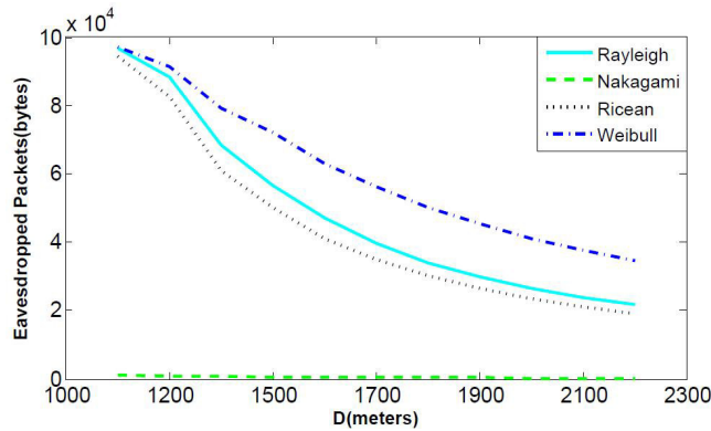
Fig. 5: Eavesdropping rate with different fading channels
