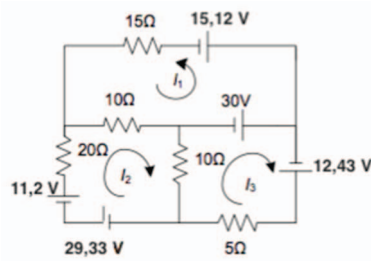
Figure 2: Electrical circuit solved in Task 2.
