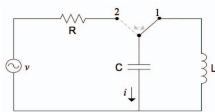
Figure 1: RLC circuit analyzed in Task 1.
