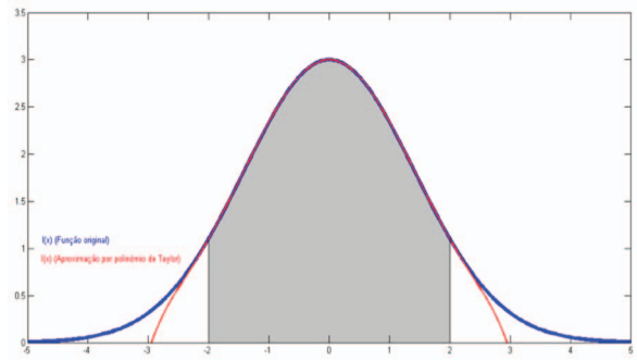
Figure 4: Numerical Integration.
