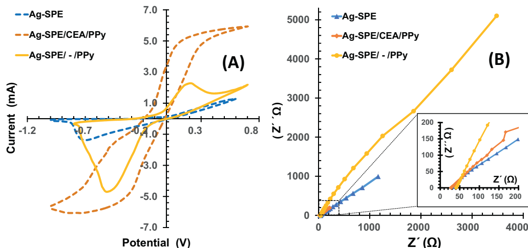
Fig. 3. Electrochemical CV (A) and EIS (B) responses of the different stages of Ag/SPE modification, evaluated in 1.0 mM Ru^{3+} , in buffer, pH 7.2.
