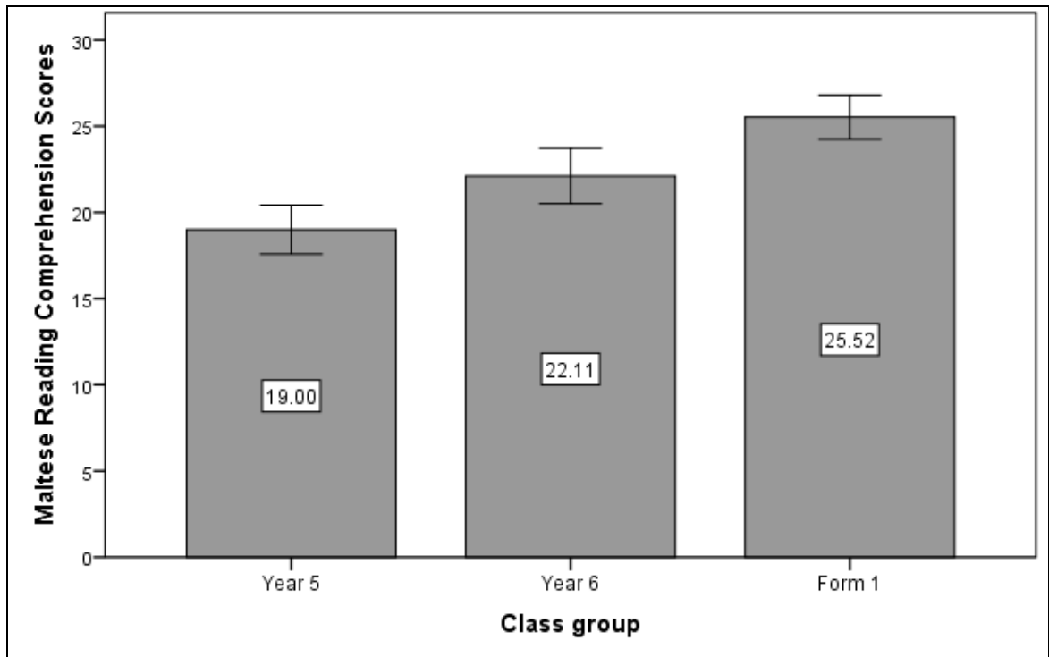
Figure 2: Error bar graph of the Reading Comprehension scores obtained by the three grade groups
