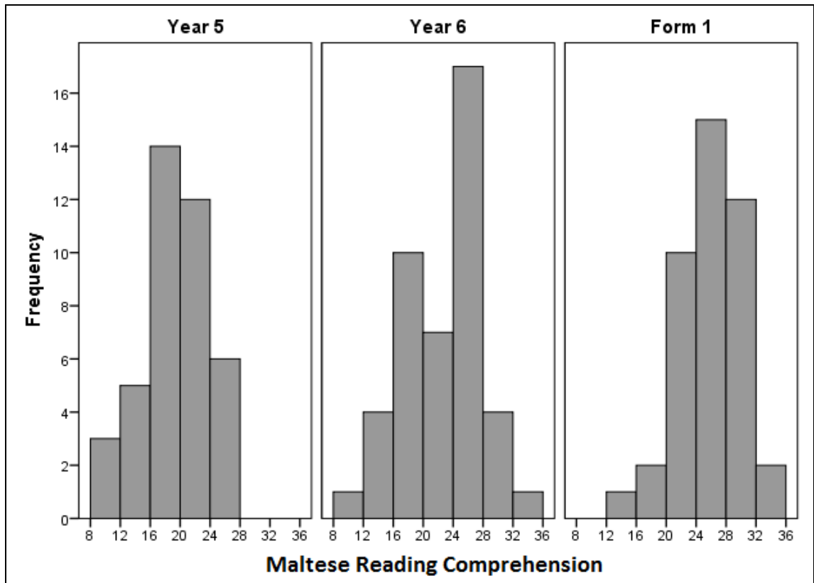
Figure 1: Histogram of distribution of Reading Comprehension scores for each grade group
