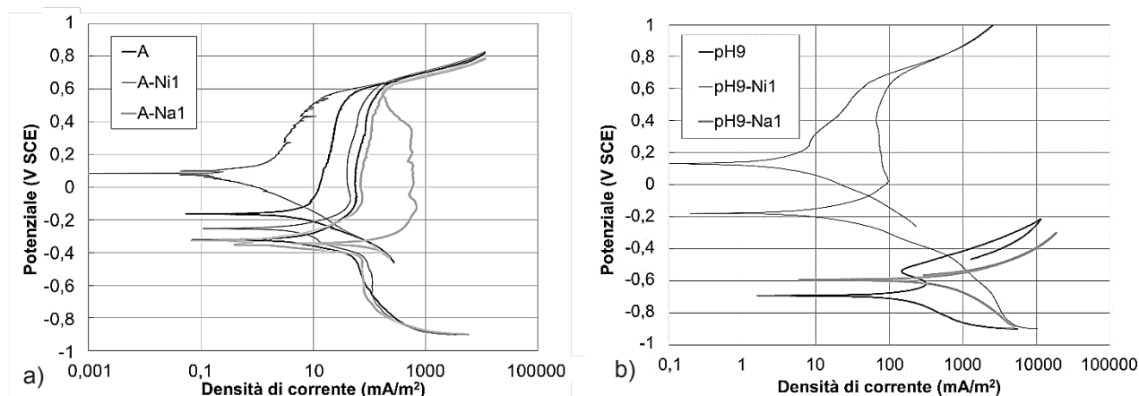
Fig. 1 – Prove potenziodinamiche effettuate in assenza di cloruri, con/senza inibitori, in soluzione alcalina (a) e a pH 9 (b) – Potentiodynamic polarization in absence of chlorides, with/without inhibitors, in alkaline solution (a) and in pH 9 solution (b)
