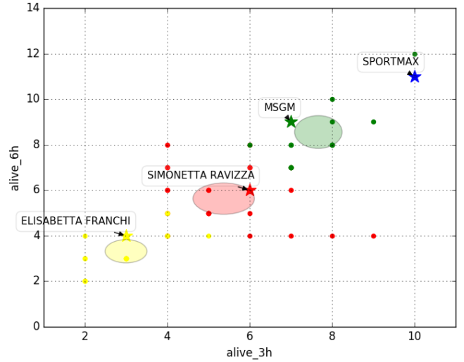
Figure 4: K-means clustering results with k=4 using the number of alive cells and the Manhattan distance as principle components; the stars represent the most representative element within each cluster, with minimal distance from the cluster centroid.
