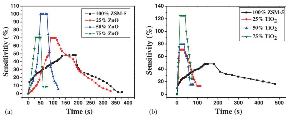
Figure 7. (a and b) Comparison of response and recovery behaviors of pure and metal oxide blended ZSM-5 composite thick film sensors as a function of time revealing the effect of metal oxide concentration. (a) ZnO/ZSM-5 at corresponding operating temperature (90, 110, 250°C) for 25, 50, 75% of ZnO, respectively, and (b) TiO 2 /ZSM-5 at corresponding operating temperature (160, 200, 115°C) for 25, 50, 75% of TiO 2 , respectively.
