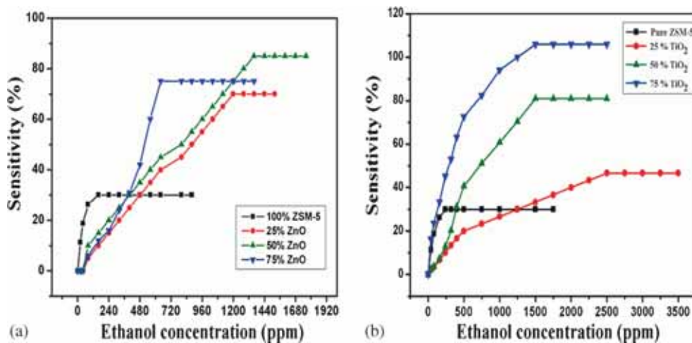
Figure 6. Comparative nature of ethanol uptake capacities of pure and metal oxide blended ZSM-5 composite thick film sensors as a function of ethanol vapour concentration. (a) ZnO/ZSM-5 at corresponding operating temperatures (90, 11 and 250°C) for 25, 50 and 75% of ZnO, respectively, and (b) TiO 2 /ZSM-5 at corresponding operating temperatures (160, 200 and 115°C) for 25, 50 and 75% of TiO 2 , respectively.
