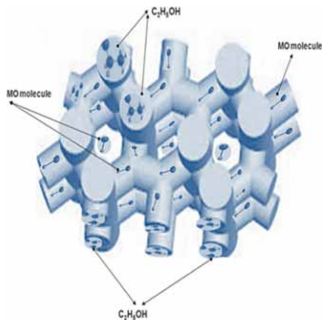
Figure 9. Schematic diagram of ZSM-5 zeolite channels with the incorporation of metal oxides (ZnO/TiO 2 ) for ethanol sensing mechanism.
