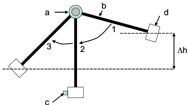
Figure 1: Schematic presentation of the Charpy pendulum impact test, showing a: the horizontal rotation axis of the pendulum, b: the stiff shaft on to which is fixed, d: the hammer. The hammer is released from a well-defined height (position 1). When the hammer has reached maximum kinetic energy (shaft in vertical position 2), the hammer strikes c: the test sample, which is positioned on a support and against the pendulum anvils (not shown). The height reached by the hammer after having broken the sample (position 3) is recorded. The difference in height between position 1 and 3 ( \Delta h ) corresponds with the difference in potential energy, and is a measure of the energy required to break the test sample.
