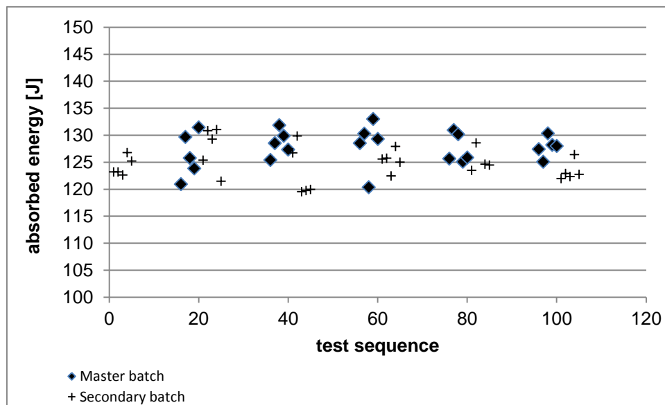
Figure 3: Absorbed energy values of 0 test pieces of ERM ® - , compared with 0 test pieces of ERM ® - ; data are displayed in the actual test sequence
