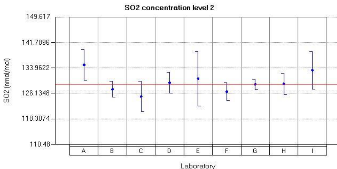
Figure 15: Reported values for SO 2 run 2.
