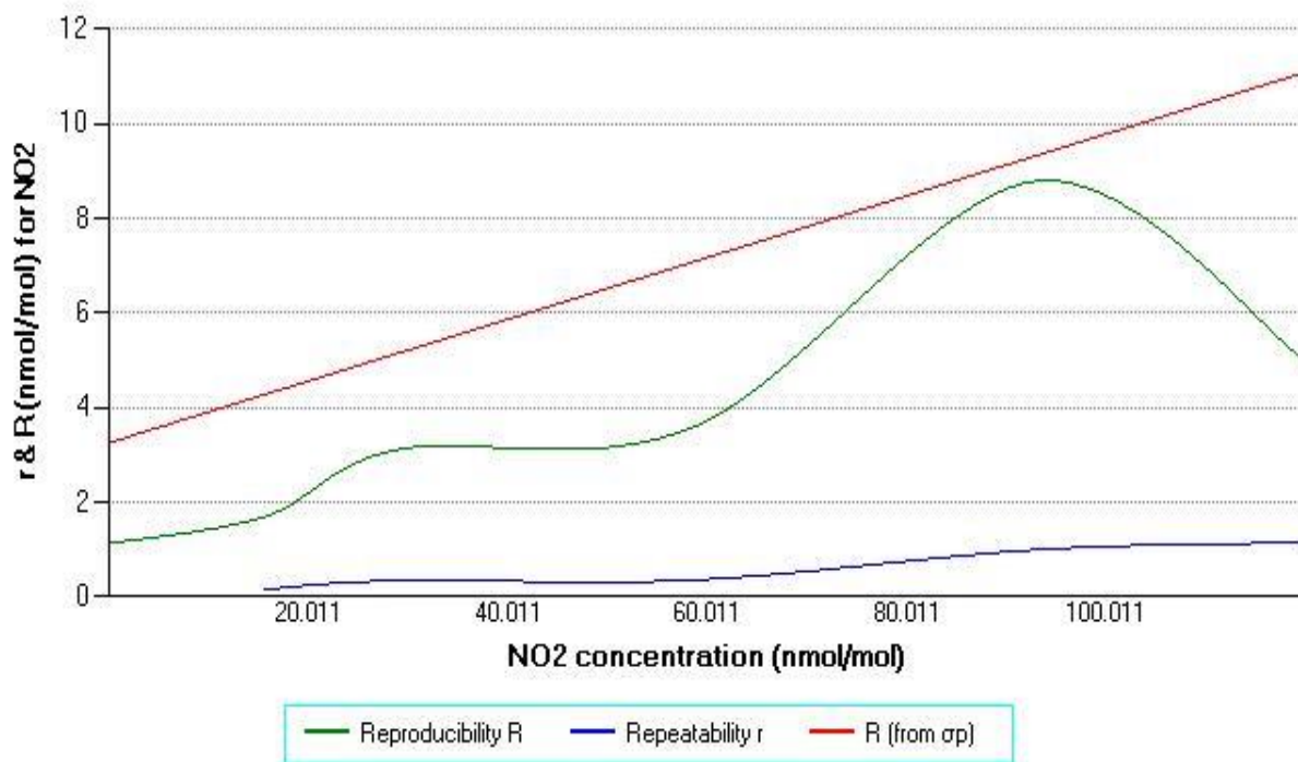
Figure 52: The R and r of NO 2 standard measurement method as a function of concentration.
