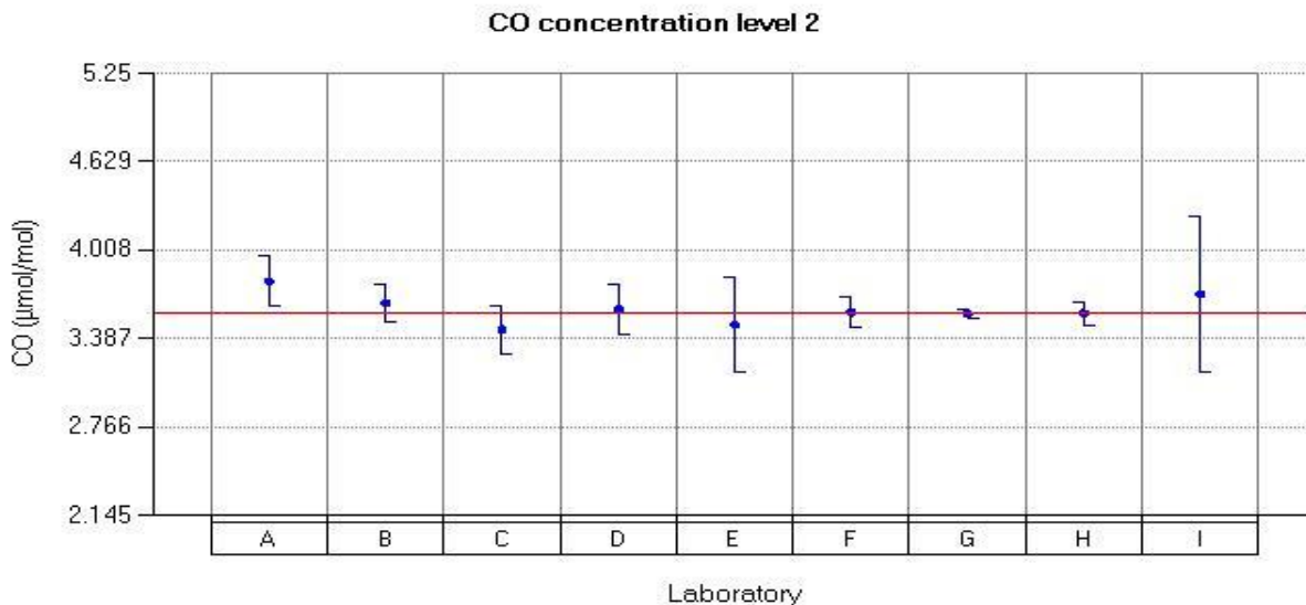
Figure 21: Reported values for CO run 2.
