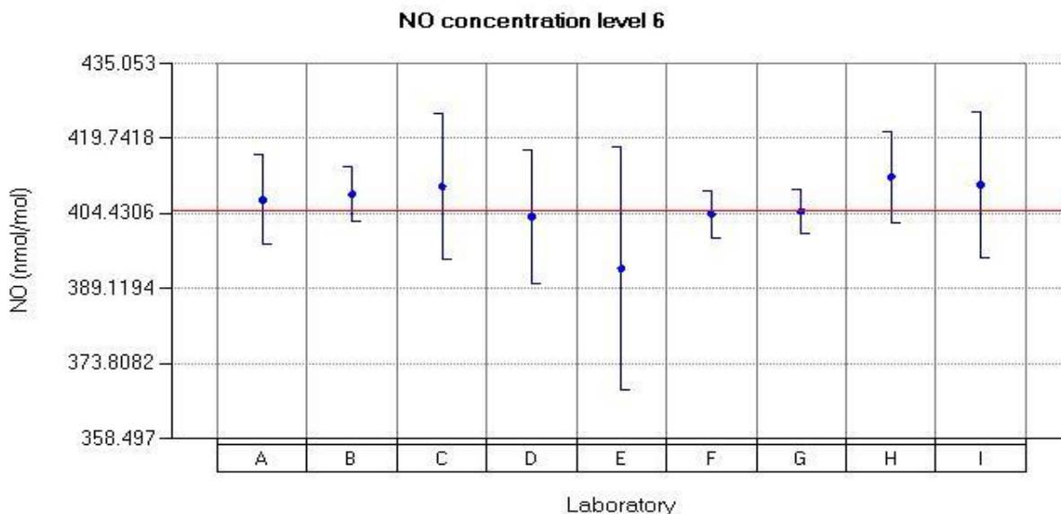
Figure 37: Reported values for NO run 6.
