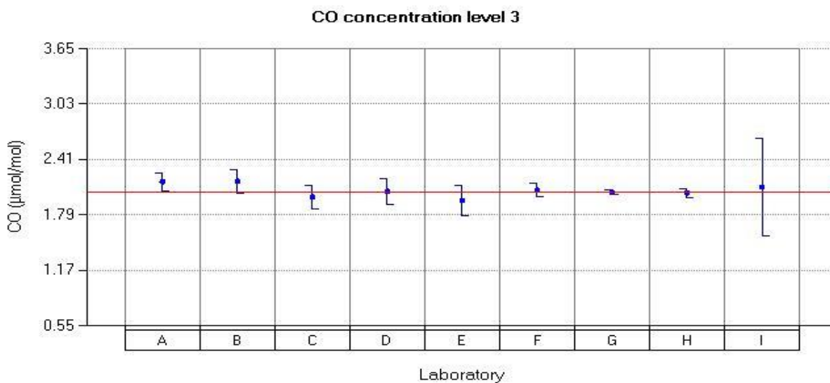
Figure 22: Reported values for CO run 3.
