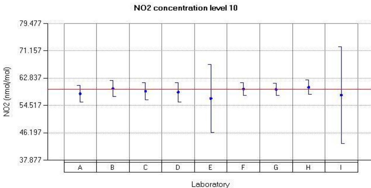
Figure 47: Reported values for NO 2 run 10.
