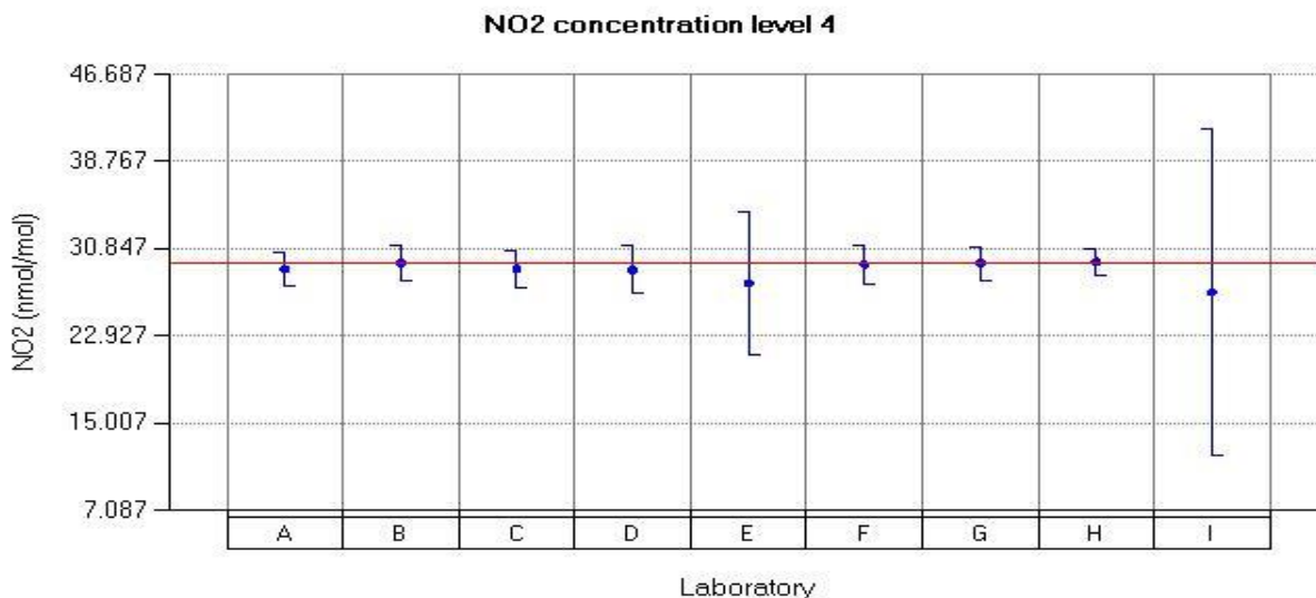
Figure 44: Reported values for NO 2 run 4.
