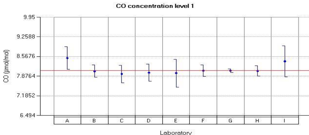
Figure 20: Reported values for CO run 1.
