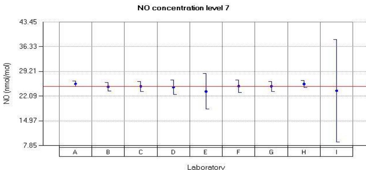
Figure 38: Reported values for NO run 7.
