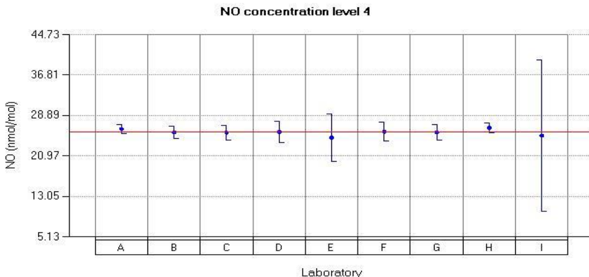
Figure 35: Reported values for NO run 4.
