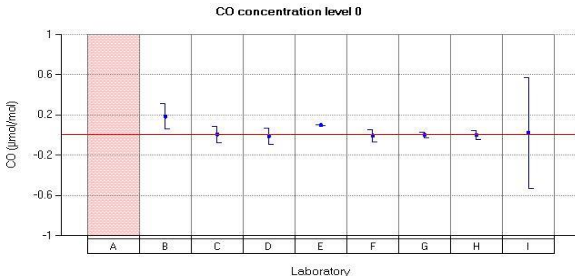
Figure 19: Reported values for CO run 0. Participant A did not report uncertainty for level 0.
