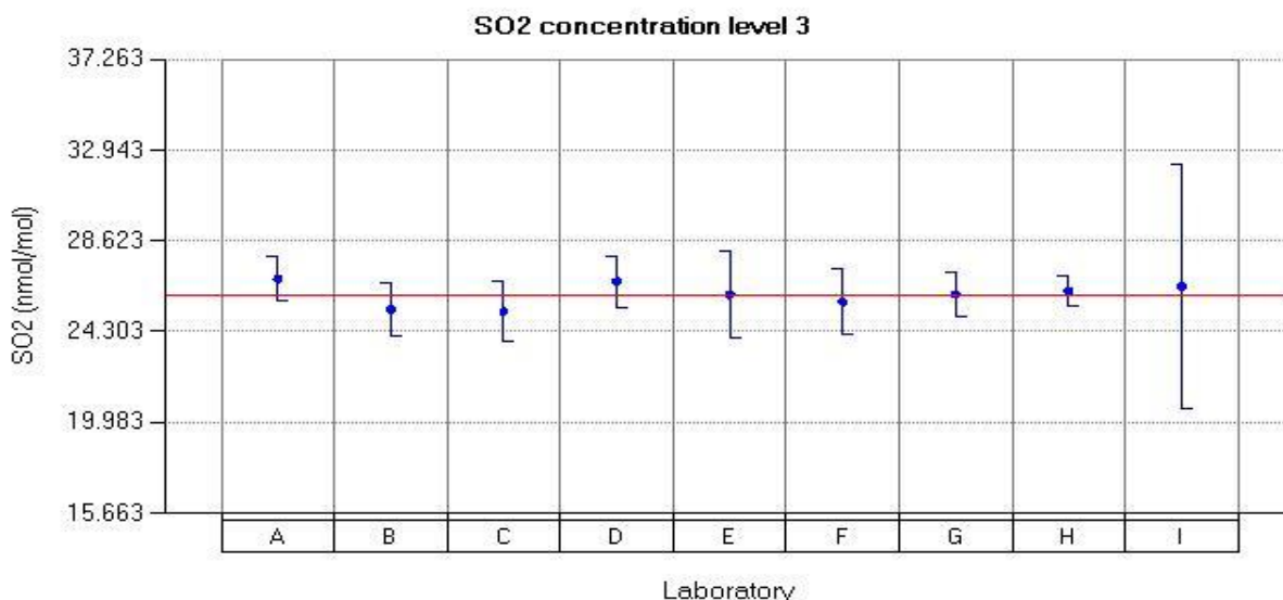
Figure 16: Reported values for SO 2 run 3.
