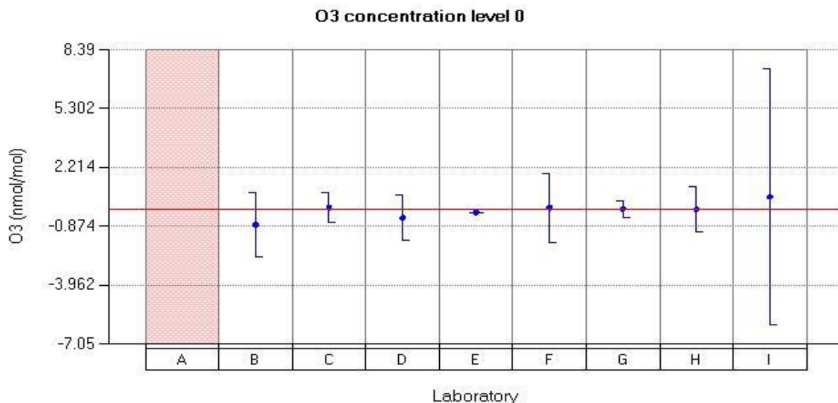
Figure 25: Reported values for O 3 run 0. Participant A did not report uncertainty for level 0.
