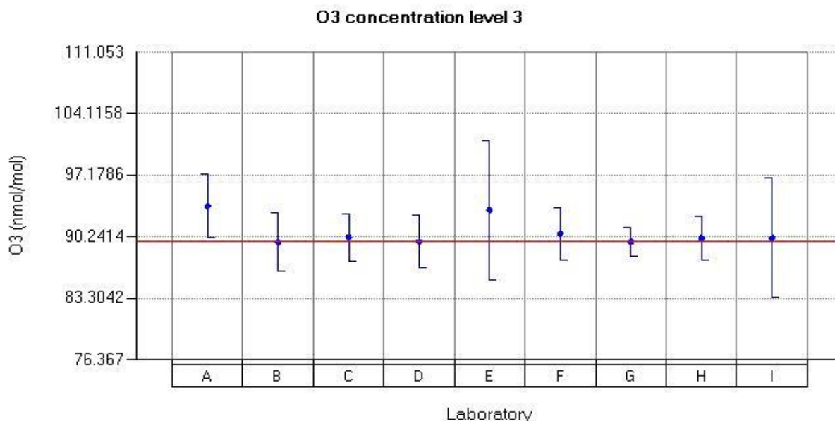
Figure 28: Reported values for O 3 run 3.
