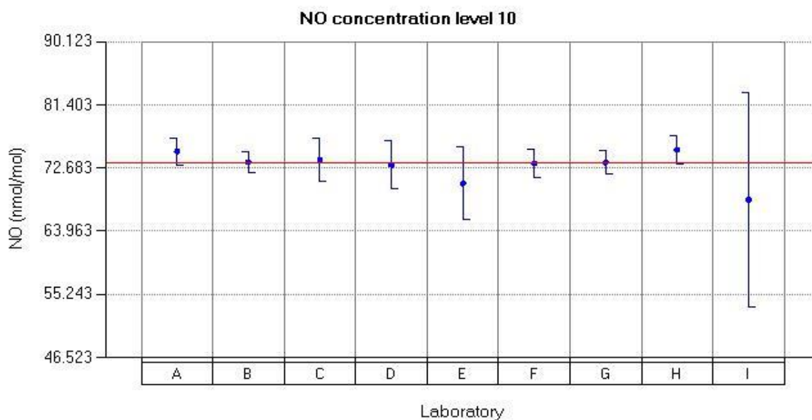
Figure 41: Reported values for NO run 10.
