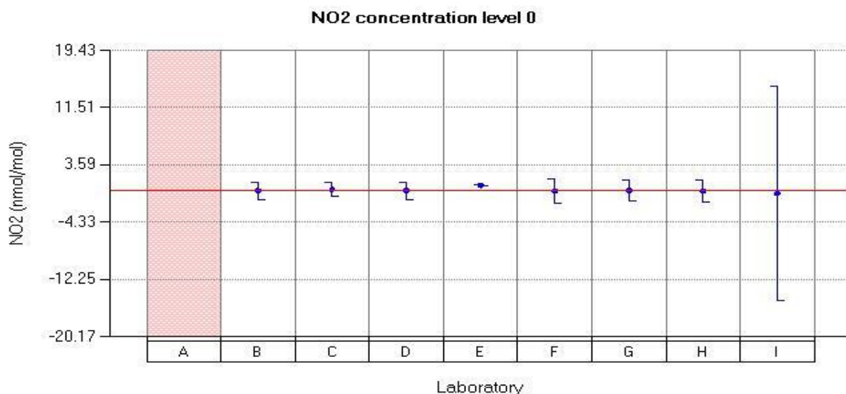
Figure 42: Reported values for NO 2 run 0. Participant A did not report uncertainty for level 0.
