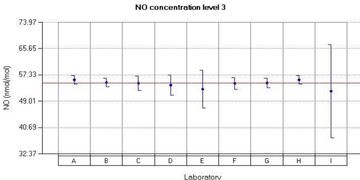
Figure 34: Reported values for NO run 3.
