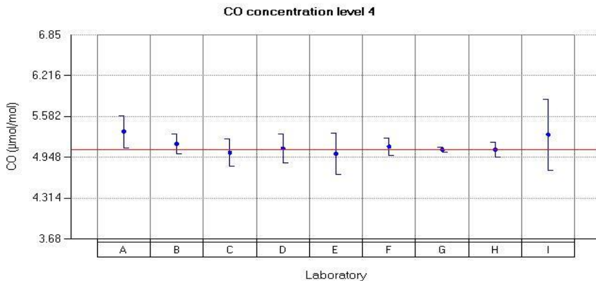
Figure 23: Reported values for CO run 4.
