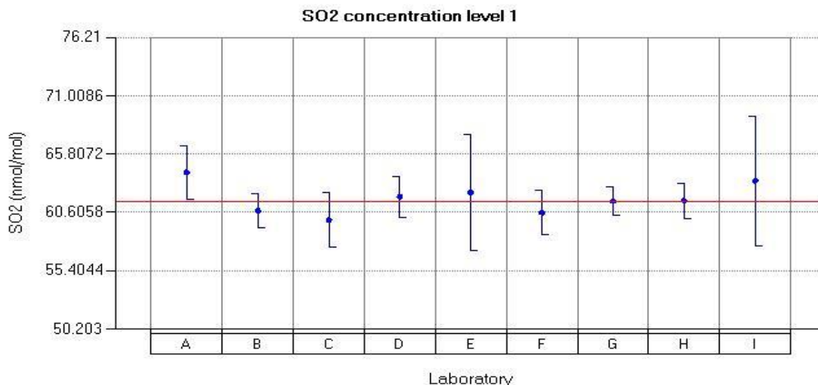
Figure 14: Reported values for SO 2 run 1.
