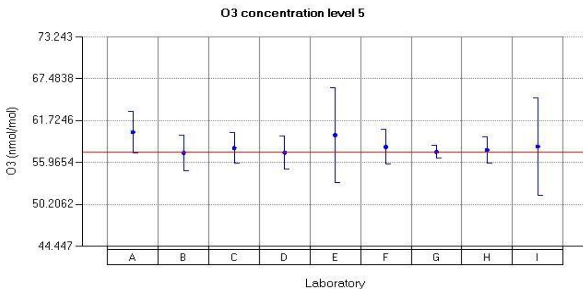
Figure 30: Reported values for O 3 run 5.
