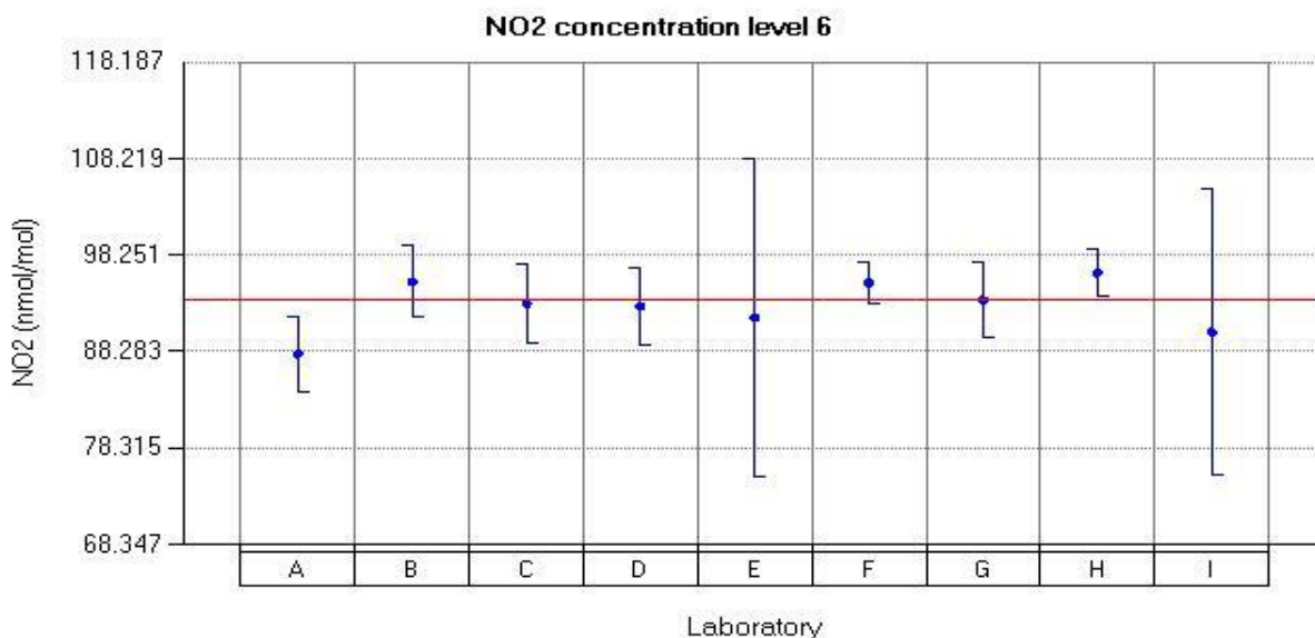
Figure 45: Reported values for NO 2 run 6.
