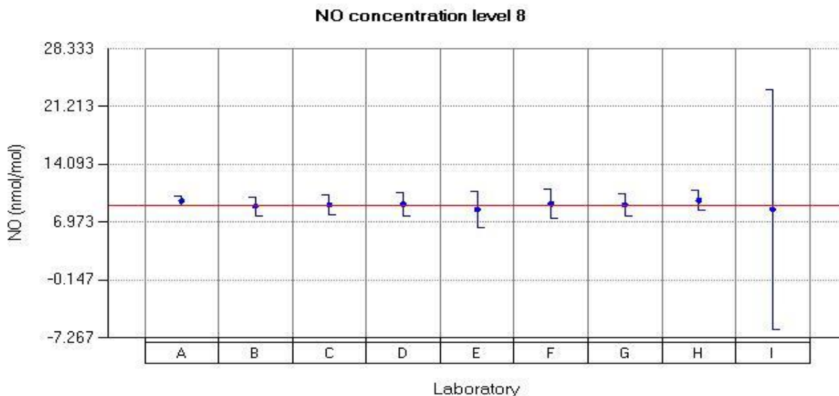
Figure 39: Reported values for NO run 8.
