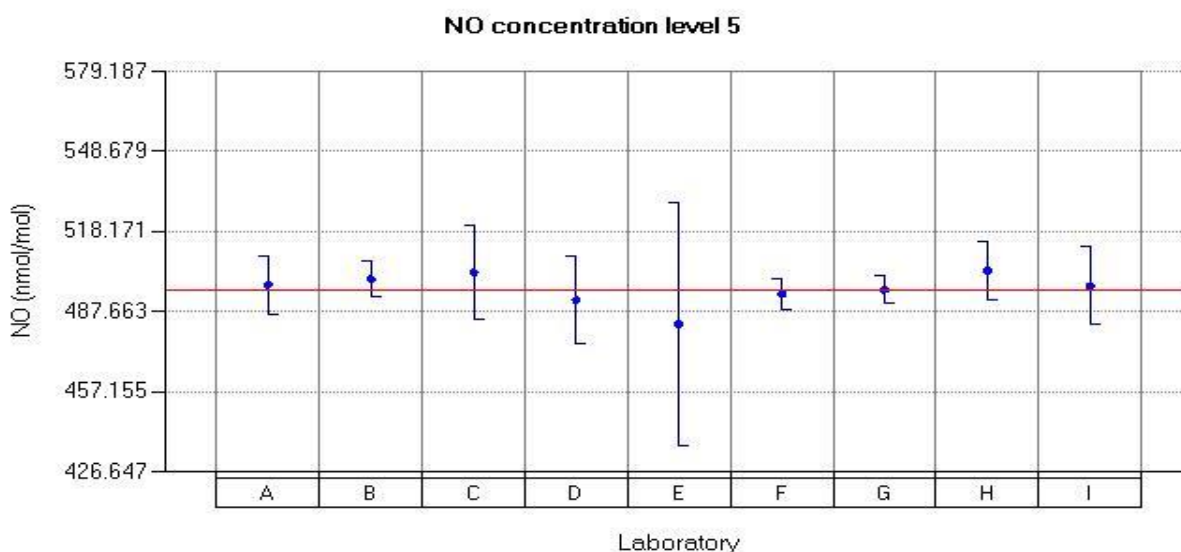
Figure 36: Reported values for NO run 5.
