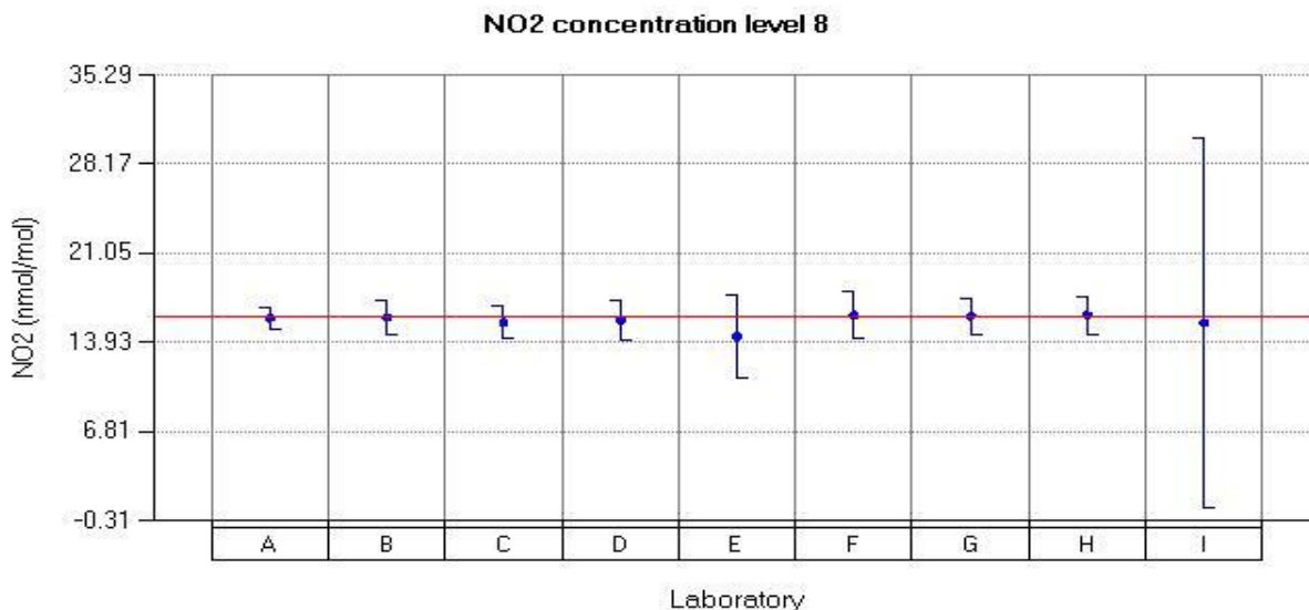
Figure 46: Reported values for NO 2 run 8.
