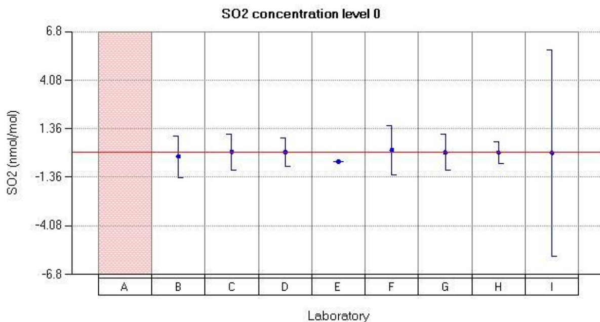
Figure 13: Reported values for SO 2 run 0. Participant A did not report uncertainty for level 0.
