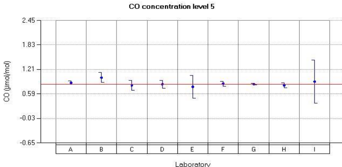
Figure 24: Reported values for CO run 5.
