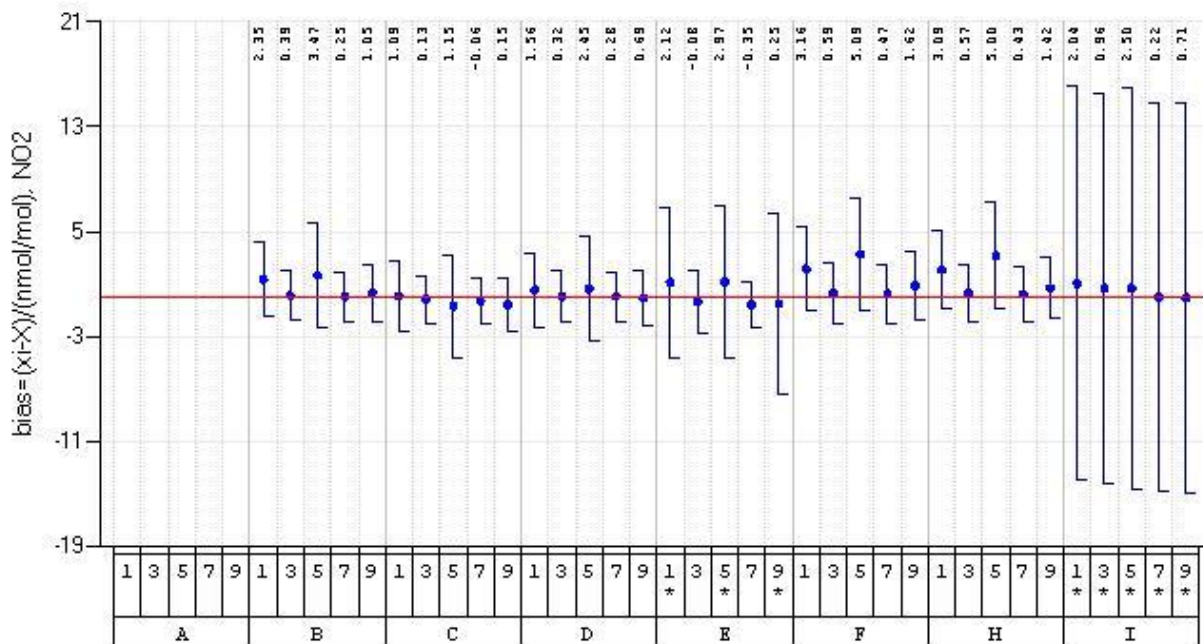
Figure 11: Bias of participant's NO 2 measurements with error bars representing expanded uncertainty for run numbers 1, 3, 5, 7 and 9. Within these test gas mixtures there is no gas phase titration to produce NO 2 (see Table 3). For each evaluation the run number together with the participants rounded run average (nmol/mol) is given. Participant A did not express uncertainties.
