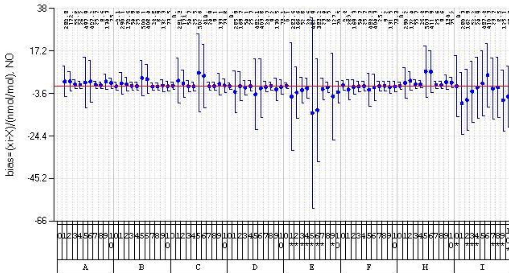
Figure 9: Bias of participant's NO measurement results
