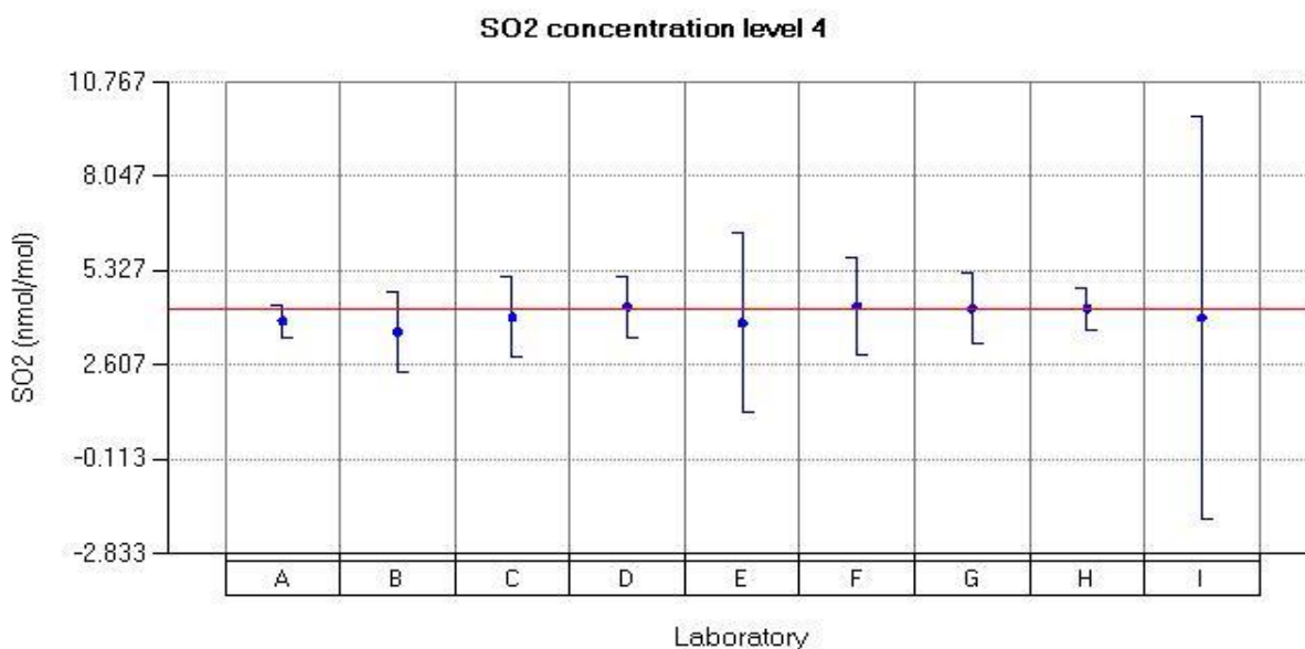
Figure 17: Reported values for SO 2 run 4.
