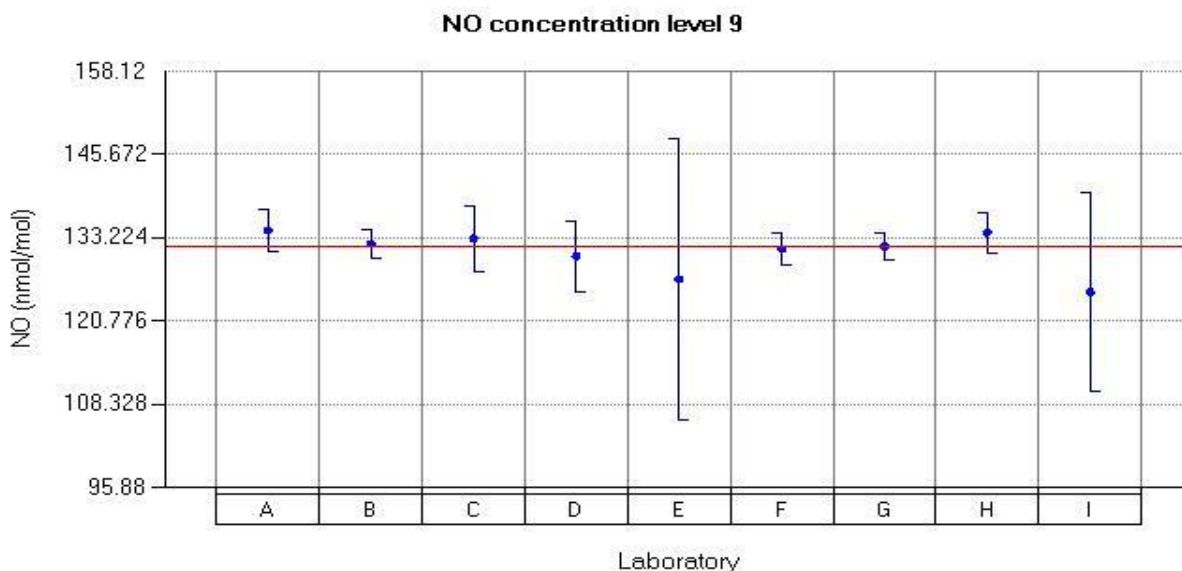
Figure 40: Reported values for NO run 9.
