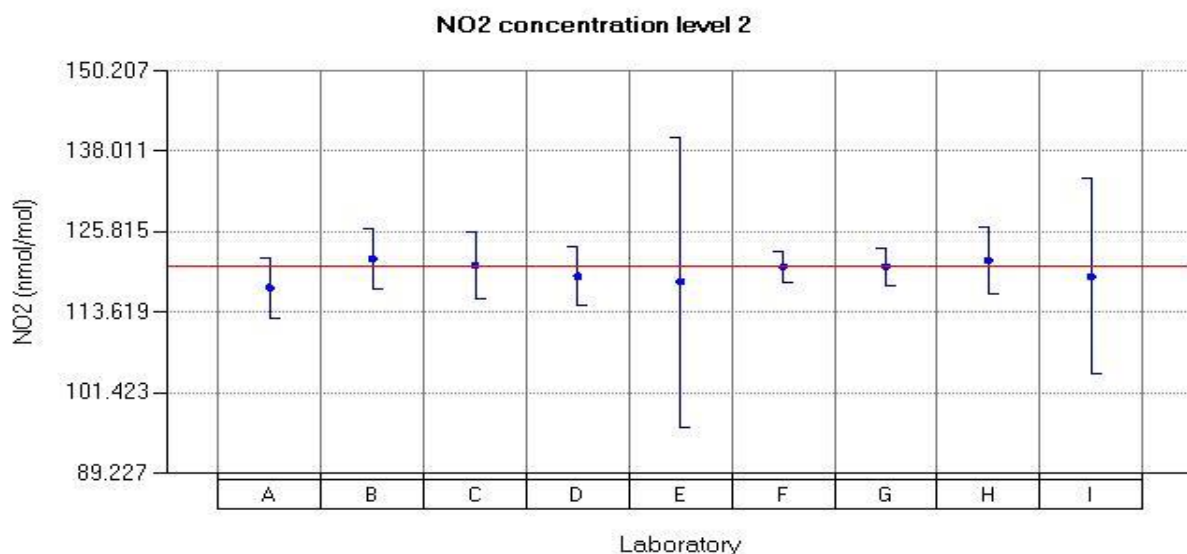
Figure 43: Reported values for NO 2 run 2.
