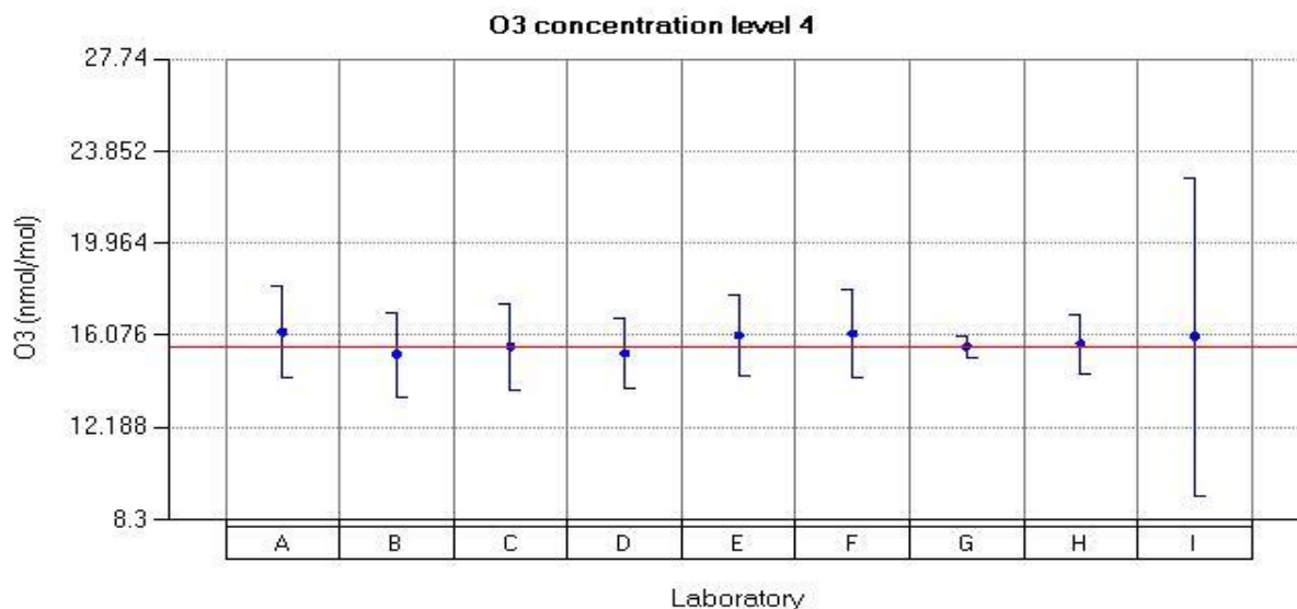
Figure 29: Reported values for O 3 run 4.
