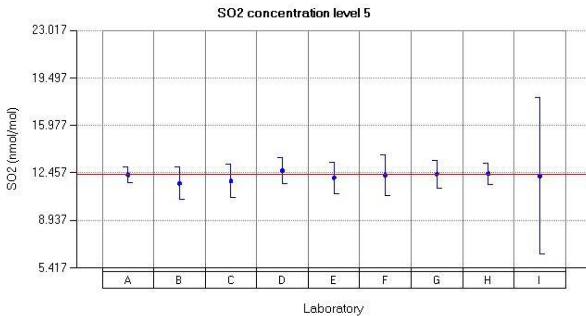
Figure 18: Reported values for SO 2 run 5.
