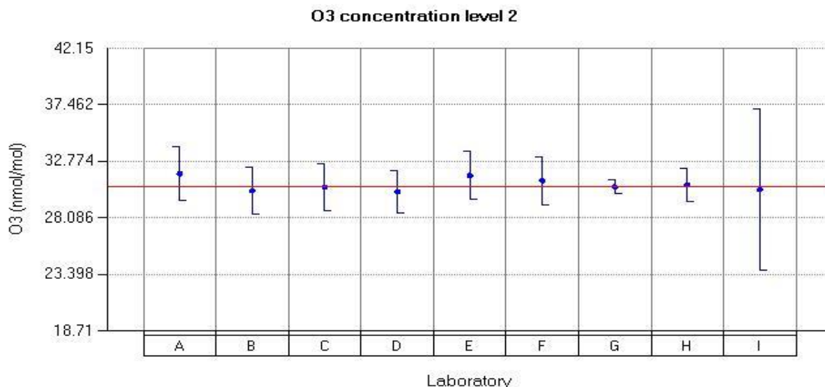
Figure 27: Reported values for O 3 run 2.
