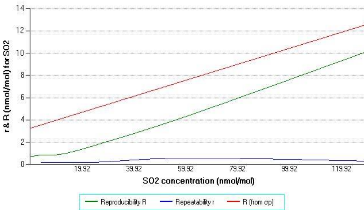
Figure 48: The R and r of SO 2 standard measurement method as a function of concentration.
