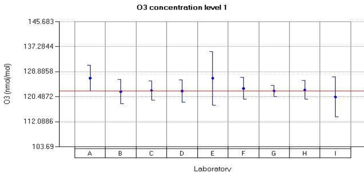
Figure 26: Reported values for O 3 run 1.
