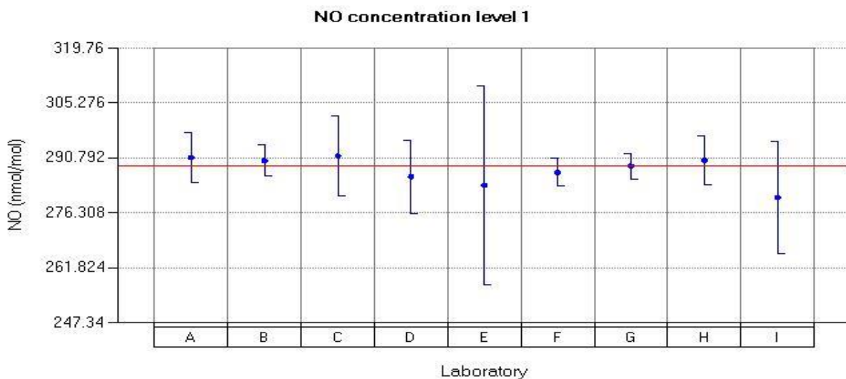
Figure 32: Reported values for NO run 1.
