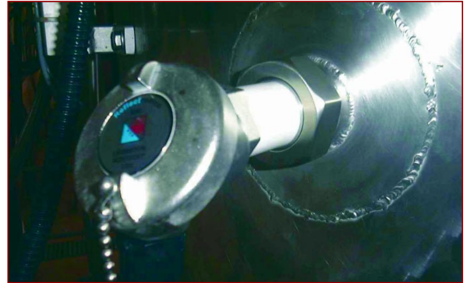
Fig. 5. Fibre optic probe installed in cheese vat.
