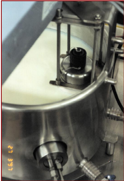
Fig. 4. Laboratory cheese vat fitted with combination of probes.
