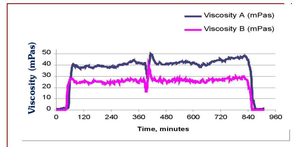
Fig. 1. Trend showing viscosity measured on-line at two points in the process during manufacture of whole-milk powder. Viscosity A was measured ex-evaporator using a vibrating rod in transverse mode. Viscosity B was measured between the concentrate heater and the atomiser using a vibrating rod in torsional mode.
