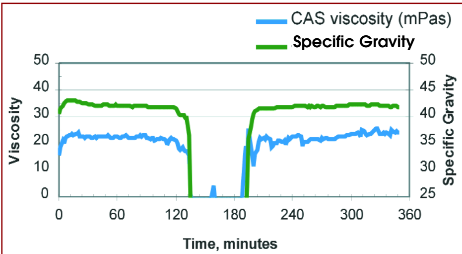
Fig. 3. Trend of viscosity measured on-line using a sliding piston sensor and specific gravity measured on-line using vibrating U-tube. The trend covers a period including some plant down-time.
