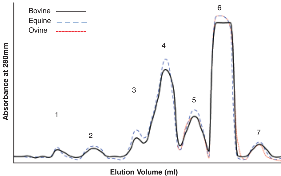
Fig. 1. The chromatographic elution profile of a low molecular weight fraction of bovine, equine and ovine follicular fluid.
