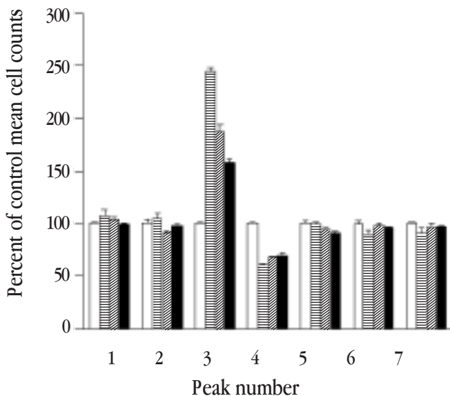
Fig. 2. Effect of various peaks from the G-25 chromatographic separation of the low molecular weight fraction of follicular fluid on granulosa cell proliferation as measured by haemocytometric cell counting. Peptide equivalent concentrations of the various peaks are shown as follows:- 0 ng ml -1 , □; 10 ng ml -1 , ▨; 100 ng ml -1 , ▩; 1000 ng ml -1 , ■.
