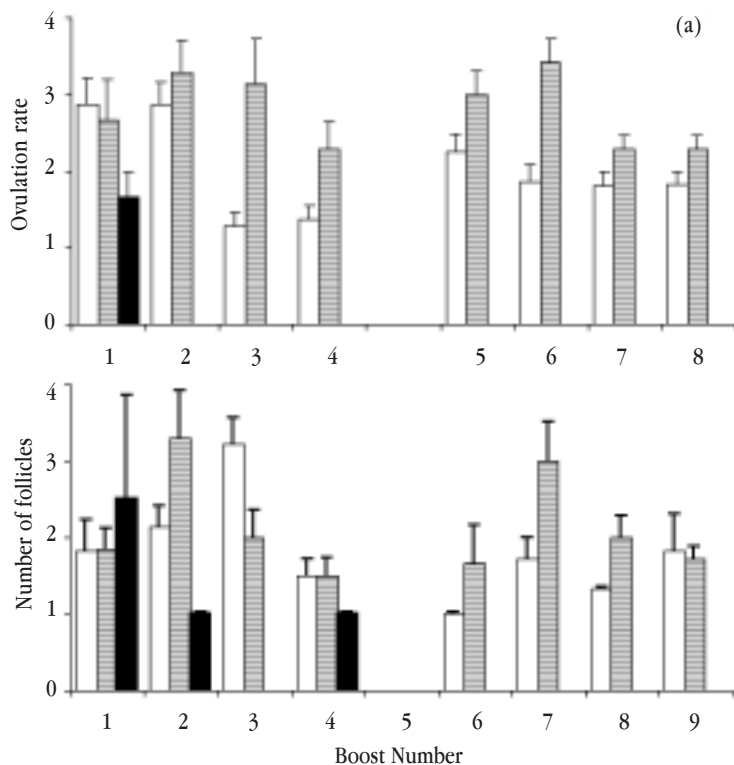
Fig.4 Effect of immunization of sheep with human serum albumin (HSA) alone (□), granulosa cell inhibitory factor GCIF-HSA (▨) or GnRH-HSA (■) over two breeding seasons on (a) ovulation rate and (b) number of follicles with a diameter >3mm per animal. Sheep immunized with GnRH were boosted only once. They did not ovulate after the first boost and had no follicles >3mm diameter after the first breeding season. Values are mean \pm s.e.m. based on all animals and 7 to 8 replicates. The overall ovulation rate was significantly different from that of HSA immunized sheep ( p < 0.01 ). The number of follicles for GCIF- and HSA-immunized sheep were not significantly different ( P > 0.05 )
