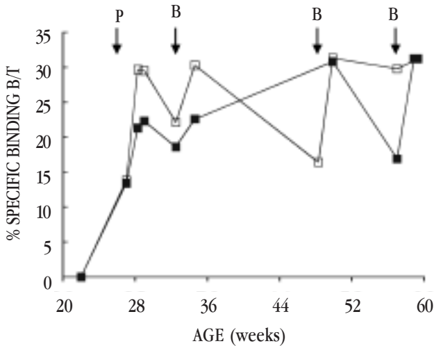
Figure 5 Percentage binding of radioiodinated 68kDa inhibin by serum from ewe lambs immunized with a partly purified preparation of bovine follicular fluid. Arrows indicate time of immunization.
