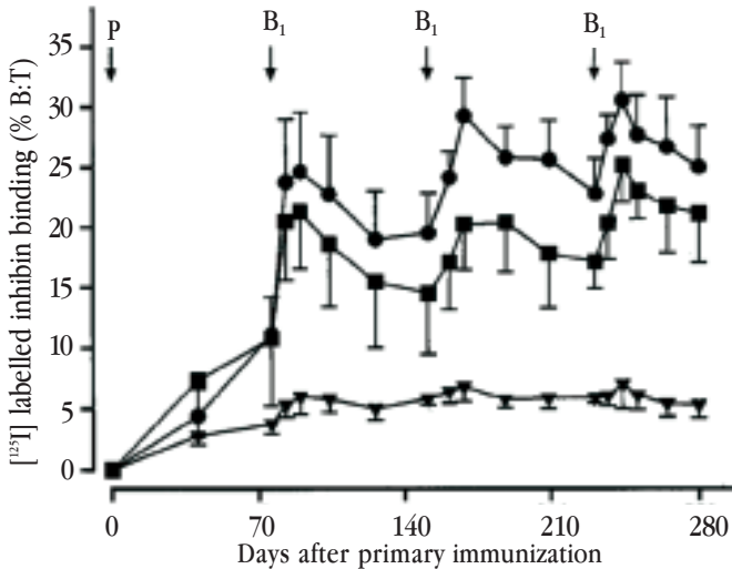
Fig. 8. Percentage binding (means±SEM) of 125 I-labelled 32kDa bovine inhibin by serum from heifers immunized against inhibin peptides (■) P1, (●) P2, and (▼) P3. Heifers were injected at intervals of 11 weeks (arrows). P: primary immunization; B1-B3: consecutive booster injections.
