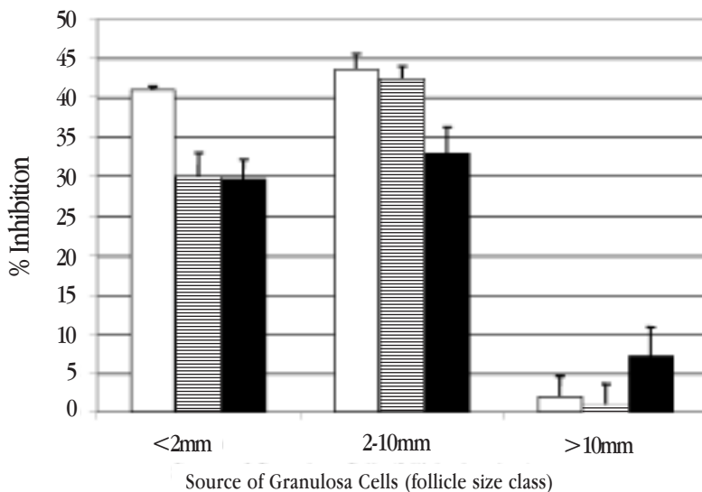
Fig.3. Effects of peak 4 isolated from a population of mixed follicles on the proliferation of granulosa cells at 0.01 ng/ml, (□); 0.10ng/ml (▨) and 1.0ng/ml, (■) monitored by [ ^3\text{H} ]thymidine incorporation into acid-precipitable material. Values are expressed as a percentage of control \pm sem.
