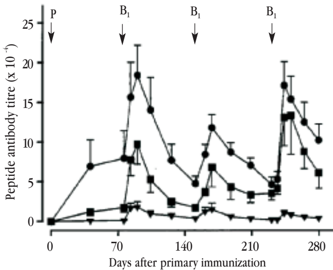
Fig. 7. Peptide antibody titres (means±SEM) in serum from heifers immunized against inhibin peptides (■) P1, (●)P2, and (▼) P3. Heifers were injected at intervals of 11 weeks (arrows). P: primary immunization; B1-B3: consecutive booster injections.
