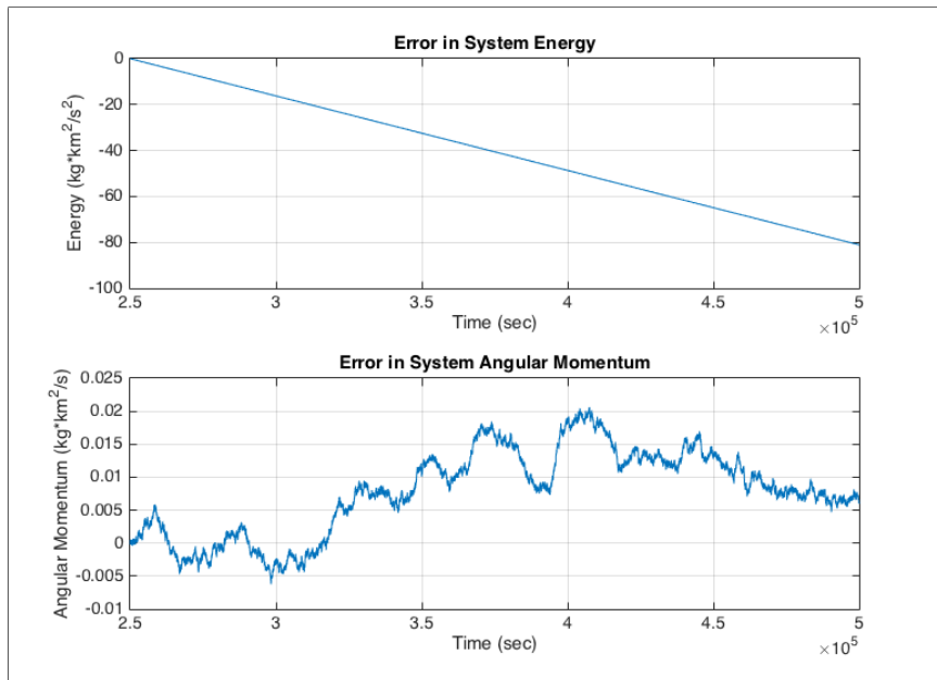
Figure 6.4: Energy and angular momentum over the last 250,000 seconds for the Euler Resting to Lagrange Resting transition. Quantities are relative to the energy and angular momentum of the system at 250,000 seconds.
