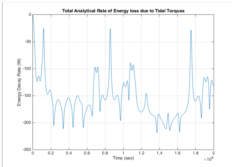
Figure 5.47: Rate of Energy decay due to Tidal Torques for the simulation of the ER to AM transition.
