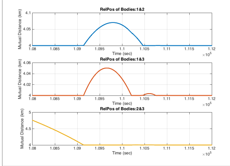
Figure 5.36: Relative body positions showing mutual body distances over the simulation for the transit of the bodies from ER to LR configuration. Notice the subsequent separation events after the impact of bodies 2 and 3. Note that the radius of each body is 2 km.
