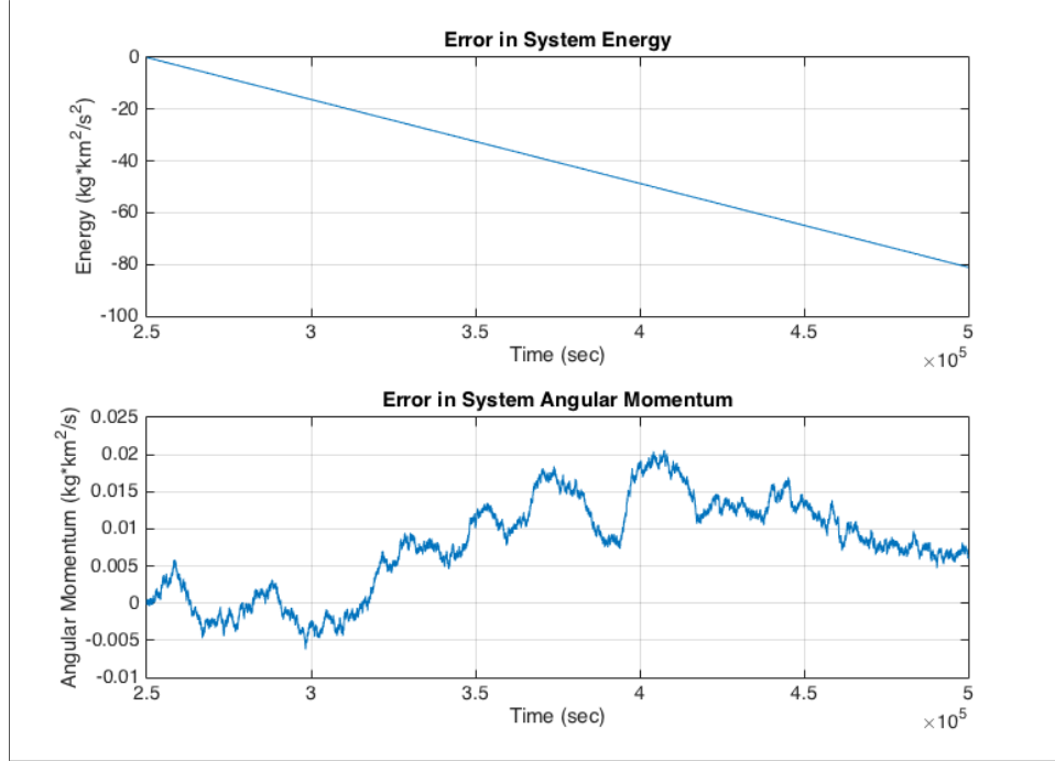
Figure 5.39: Net change in energy and angular momentum relative to the system at 250,000 seconds for the simulation of the ER to LR transition.
