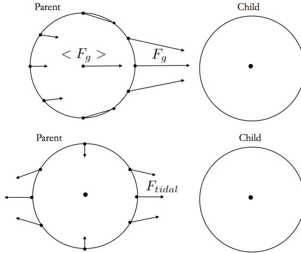
Figure 3.2: Gravity gradients cause stretching along a center of mass axis and compression along a perpendicular axis [9]. Relative to the center of mass of the Parent body, the side facing the Child body will experience a greater gravitational force towards the Child. The side facing away from the Child will experience a greater gravitational force away from the Child.
