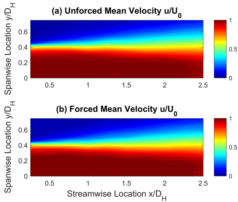
Figure 3.15: Mean velocity contours of (a) unforced and (b) forced developed flow.
