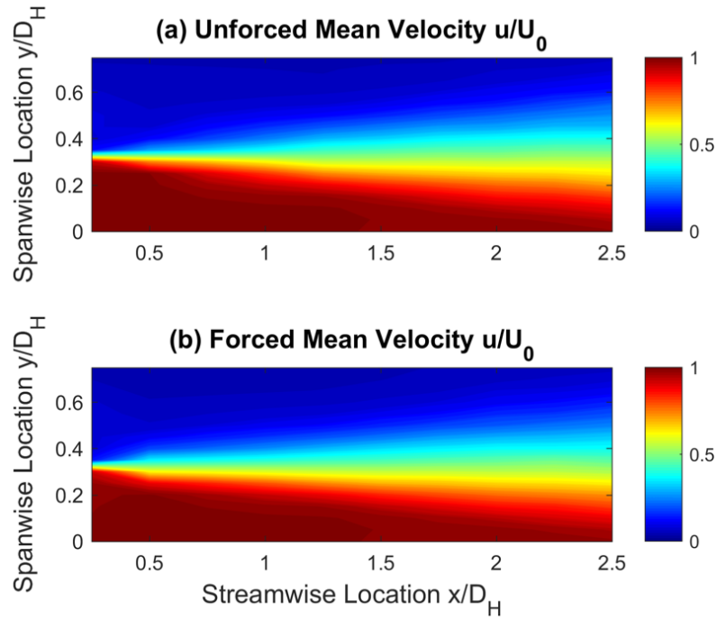
Figure 3.14: Mean velocity contours of (a) unforced and (b) forced undeveloped flow.
