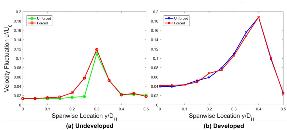
Figure 3.11: Forced and unforced spanwise distributions of velocity fluctuation at x/D_H = 0.25 for the (a) undeveloped and (b) developed flows.
