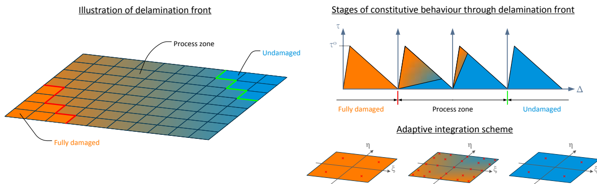
Figure 3: Illustration of the adaptive integration scheme of [16] using a Gauss-Legendre quadrature rule.
