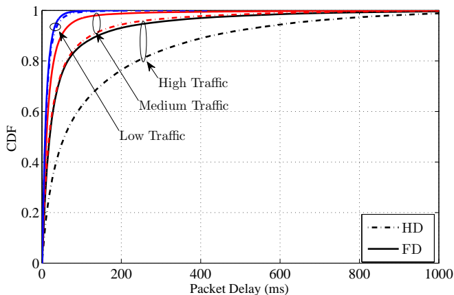
Fig. 6. CDF of the transmission delay with 5 dB wall loss for different traffic profiles.
