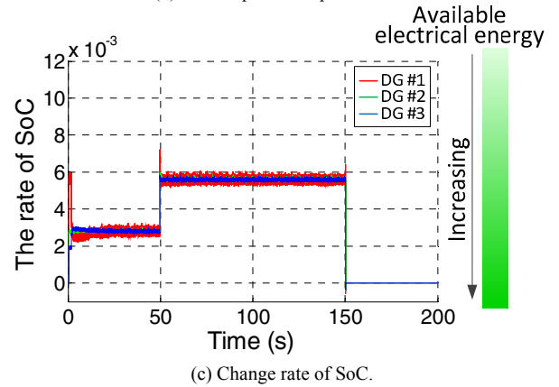
Fig. 7. Experimental results with the proposed dynamic consensus algorithm-based coordinated control.
