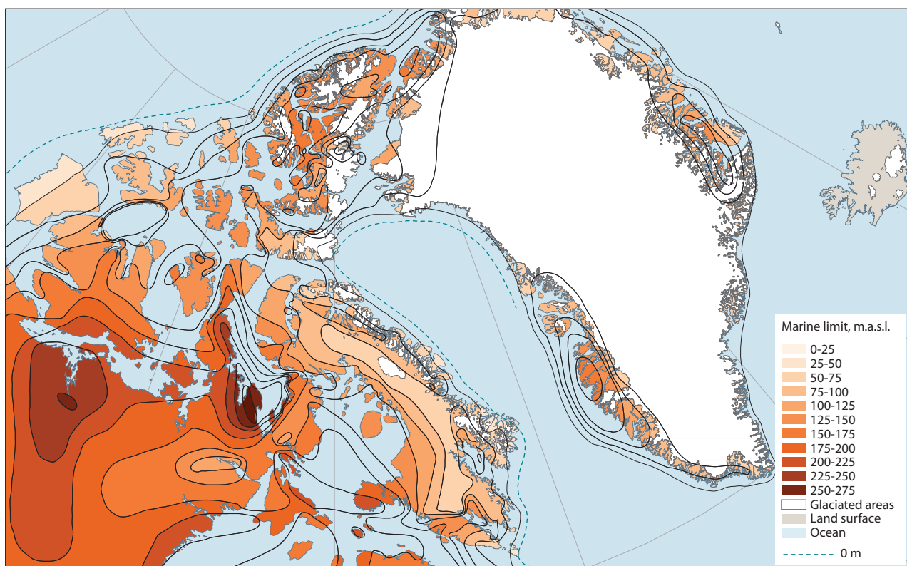
Figure 10.9 Deglacial upper marine limit (maximum relative sea level in meters above present sea level, m.a.s.l.) in the BBDS region (modified from Dyke et al., 2005). In the absence of detailed local observations, the upper marine limit can be used as a first indicator of risk in permafrost regions. At elevations below the upper marine limit, fine-grained ice-rich deposits may be encountered, depending on local depositional history and ground temperature regime. Contour interval is 25 m (the 0 m contour is dashed).
