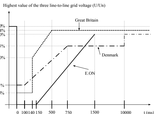
Fig. 1. Limit curves for the voltage to allow generator disconnection Tsili and Papathanassiou (2009).
