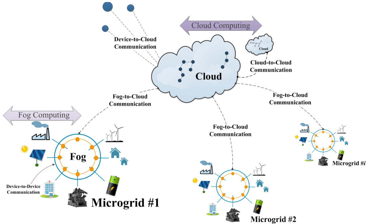
Fig. 3. Micro-grid considered as a fog domain
