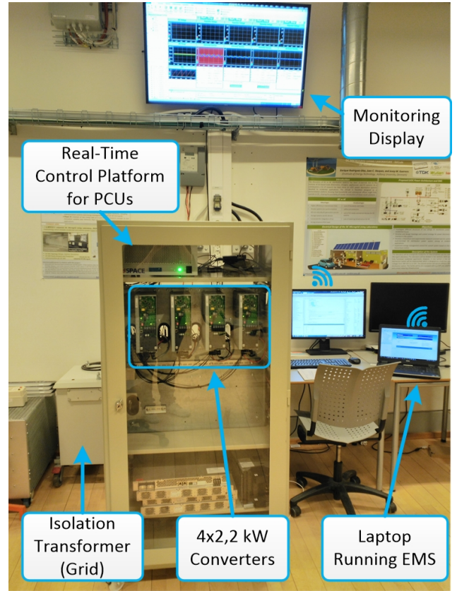
Figure 6: Experimental test-bed
