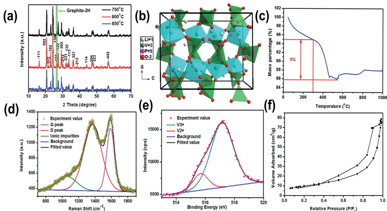
Fig. 5 Structure characterizations. (a) XRD patterns of the samples synthesized with different calcination temperature, LVP/HC-1: 750 °C, LVP/HC-2: 800 °C, LVP/C-3: 850 °C. (b) The crystal structure of LVP. (c) TG curves of the LVP/HC-2 sample in air atmosphere. (d) Raman spectrum of the LVP/HC-2 sample, the D and G peaks are deconvoluted by three-Gaussian peaks. (e) Two-Gaussian peaks fitting deconvolution of high resolution XPS V_{2p} spectrum for LVP/HC-2 sample. (f) The nitrogen adsorption–desorption isotherms of the LVP/HC-2 sample.
