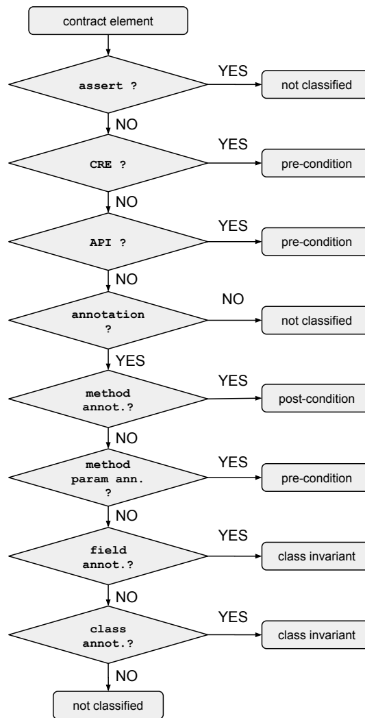
■ Figure 1 Contract element classification algorithm.
