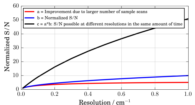
Figure 6. Spectral signal-to-noise ratio (S/N) as a function of resolution. The improvement due to lower resolution (blue line) and averaging over larger number of spectra in the same time frame (red line) and the resulting relative S/N from both effects (black line), normalized to the S/N at 0.02\text{ cm}^{-1} .
