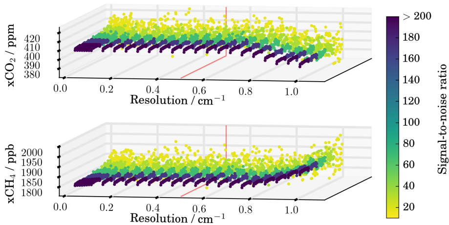
Figure 5. Retrieved xCO 2 and xCH 4 from cropped interferograms with different resolutions and different levels of white noise ( z axis and colour bar) added to the spectra.
