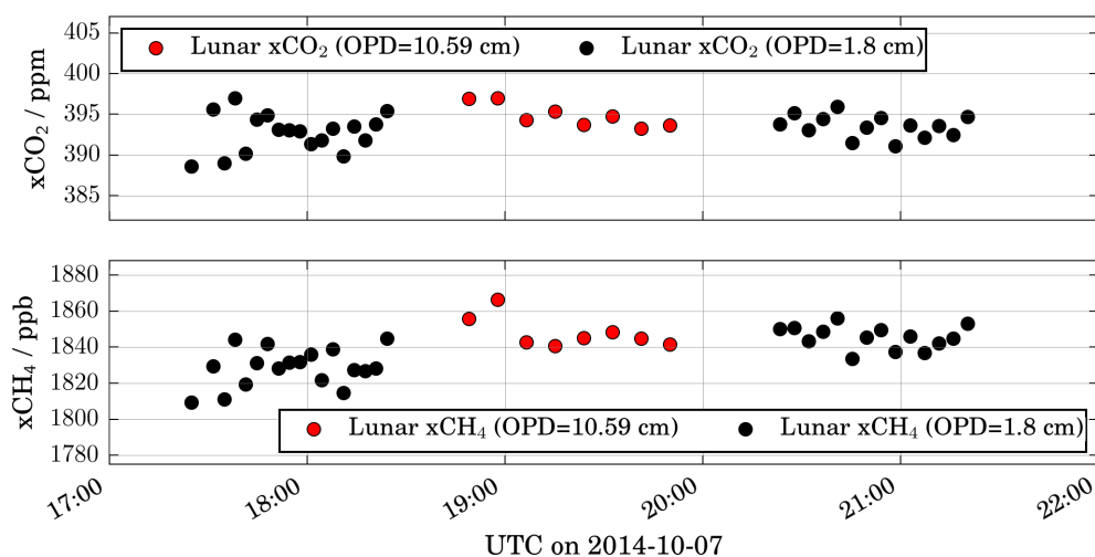
Figure 8. Comparison of retrieved xCO 2 and xCH 4 for different resolutions from low (OPD = 1.8 cm \hat{=} 0.5 cm -1 , black) and higher (OPD = 10.59 cm \hat{=} 0.085 cm -1 , red) resolution measurements on 7 October 2014.
