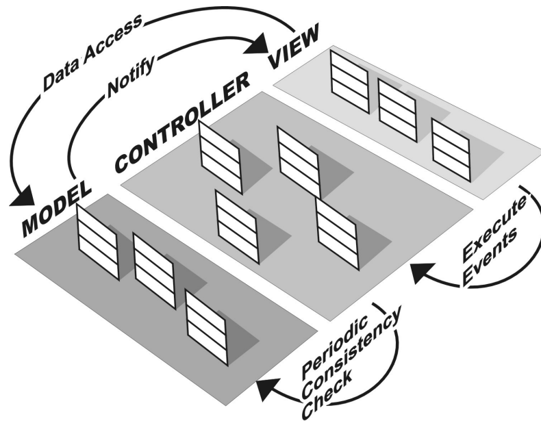
Figure 3 Coping with vulnerability of the PMIS to dynamic change of requirements through introducing three separate intersecting tiers in MARSHAL
