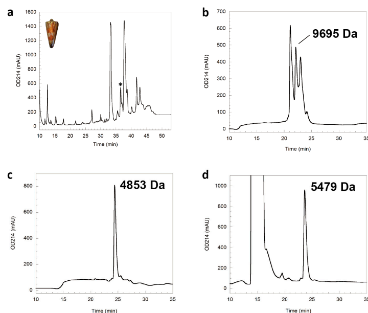
Figure 1. Purification and identification of O-conotoxin GeXXVIIA from Conus generalis . (a) Purification of crude venom extracted from C. generalis (shown in inset) on a ZORBAX C18 semi-preparative column. The asterisk indicates the fraction containing GeXXVIIA. The elution gradient is 0–50% Buffer B for 0–50 min with a flow rate of 0.5 mL/min. (b) Analytical scale purification of the GeXXVIIA-containing fraction from panel (a) on a C18 reverse-phase analytical column. The peak with a molecular mass of 9695 Da is that of GeXXVIIA. The elution gradient is 10–30% Buffer B for 0–10 min and 30–39% Buffer B for 10–37 min with a flow rate of 0.5 mL/min. (c) Purification of the reduced GeXXVIIA after being treated with DTT on a C18 reverse-phase analytical column. The elution gradient is 10–45% Buffer B for 0–35 min with a flow rate of 0.5 mL/min. (d) Purification of the GeXXVIIA peptide after being alkylated with NEM on a C18 reverse-phase analytical column. The elution gradient is the same as that of panel (c).
