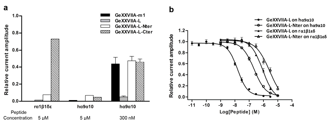
Figure 5. Antagonist potencies of GeXXVIIA-L and GeXXVIIA-L-Nter at the rodent \alpha 1\beta 1\epsilon\delta and human \alpha 9\alpha 10 nAChRs. (a) Inhibition of ACh-evoked peak current amplitude mediated by r\alpha 1\beta 1\epsilon\delta and h\alpha 9\alpha 10 nAChRs by GeXXVIIA-m1, GeXXVIIA-L, GeXXVIIA-L-Nter, and GeXXVIIA-L-Cter at 5 \mu M ( n = 1 oocyte) and 300 nM ( n = 3 –7 oocytes) peptide concentrations. Error bars indicate SEM. (b) Concentration-response curves obtained for GeXXVIIA-L and GeXXVIIA-L-Nter inhibition of r\alpha 1\beta 1\epsilon\delta and h\alpha 9\alpha 10 nAChRs expressed in Xenopus laevis oocytes. Full-length GeXXVIIA-L exhibits potent inhibitory activity at h\alpha 9\alpha 10 receptors with an IC 50 of 16.2 \pm 1.4 nM ( n = 4 –8 oocytes for each data point).
