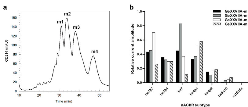
Figure 3. Preparation and nAChR-inhibitory activities of the monomeric isomers of GeXXVIIA. (a) Separation of four GeXXVIIA monomeric isomers (m1, m2, m3, and m4) refolded in vitro on a C18 reverse-phase analytical column. The elution is isocratic at 22% Buffer B with a flow rate of 0.5 mL/min. The molecular masses of these four isomers are the same, 4807 Da, indicating that two disulfide bonds are formed in each isomer. (b) The inhibition of 5 \mu M GeXXVIIA-m1, -m2, -m3, and -m4 on ACh-evoked peak current amplitude mediated by h\alpha 3\beta 2 , h\alpha 3\beta 4 , h\alpha 7 , h\alpha 4\beta 4 , h\alpha 4\beta 2 , h\alpha 9\alpha 10 , and rodent (r) \alpha 1\beta 1\epsilon\delta nAChRs ( n = 1 oocyte for each nAChR subtype).
