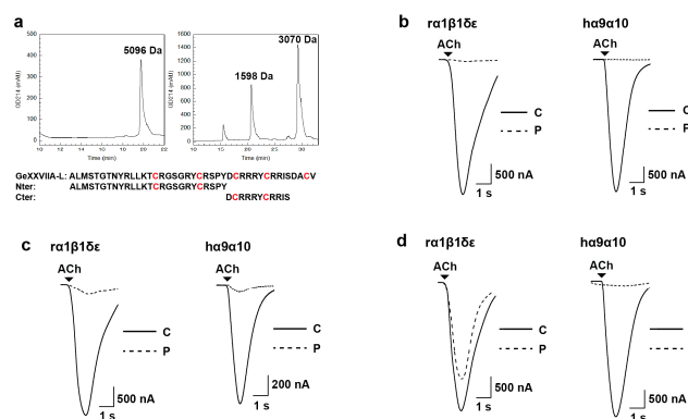
Figure 4. Preparation and nAChR-inhibitory activities of the linear GeXXVIIA and its N- and C-terminal fragments. (a) Left panel: Preparation of the linear peptide of GeXXVIIA (GeXXVIIA-L) alkylated with IAA on a C18 reverse-phase analytical column. Its molecular mass is 5096 Da. The elution gradient is 15–37% Buffer B for 0–22 min with a flow rate of 0.5 mL/min. Right panel: Two fragments were obtained after the digestion of GeXXVIIA-L by Asp-N protease. The elution gradient is 5–38% acetonitrile for 0–33 min with a flow rate of 0.5 mL/min. The N-terminal (Nter) and C-terminal (Cter) fragments of GeXXVIIA-L have a molecular mass of 3070 Da and 1598 Da, respectively. Below are the sequences of GeXXVIIA-L, Nter and Cter peptides, with the IAA-blocked Cys residues shown in red. (b–d) Superimposed ACh-evoked currents mediated by \text{r}\alpha 1\beta 1\epsilon\delta and \text{h}\alpha 9\alpha 10 nAChRs in the absence (C, control) and the presence of 5 \mu M different GeXXVIIA peptides (P). Arrows ( \blacktriangledown ) indicate ACh application. The peptides are GeXXVIIA-L (b), GeXXVIIA-L-Nter (c), and GeXXVIIA-L-Cter (d).
