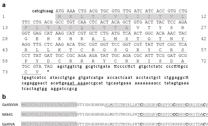
Figure 2. cDNA sequence of O-GeXXVIIA. (a) The cDNA sequence of GeXXVIIA and the cDNA-encoded precursor sequence. The coding region of cDNA is shown in capital letters. The signal peptide sequence is shadowed, and the mature peptide sequence is underlined. Between the signal sequence and mature toxin region is the pro-peptide region. * represents the stop codon. (b) Alignment of the precursor sequences of GeXXVIIA, Mik41 [19], and GeXIVA [20]. Mature toxin sequences are underlined with the Cys residues highlighted in bold.
