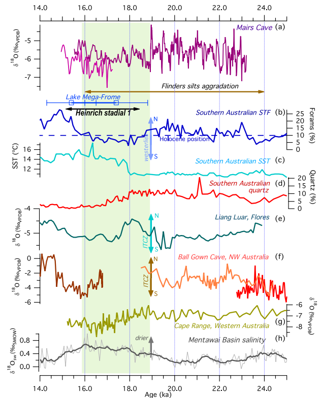
Figure 6. The Mairs Cave \delta^{18}\text{O} record (a) compared with the foraminifera record (b, c) and the quartz record (d) in marine core MD03-2611 from the Murray Canyons region, southern Australia (De Deckker et al., 2012). Speleothem records from Liang Luar, Flores (Ayliffe et al., 2013) (e); Ball Gown Cave, Western Australia (Denniston et al., 2013a) (f); and C126 Cave in Cape Range, also in Western Australia (Denniston et al., 2013b) (g). Reconstructed salinity from marine core SO189-39KL from the northern Mentawai Basin, Indonesia (h).
