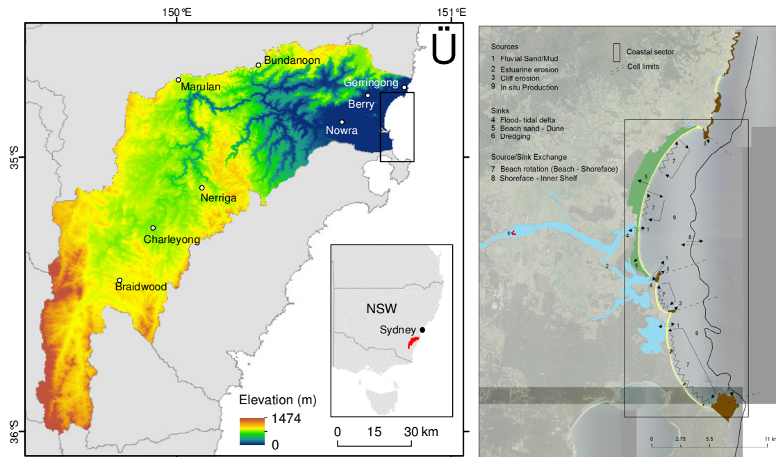
Fig.1: Shoalhaven catchment and Sediment budget compartment scheme
