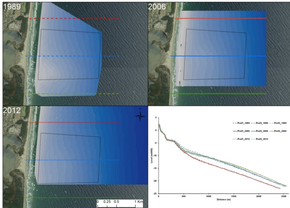
Fig.3: Bathymetric variation between 1989, 2006 and 2012. Areas used for volume calculation are shown in black outline polygon. Nearshore profiles are shown in red, blue and green lines and plotted on the bottom right corner graph.
