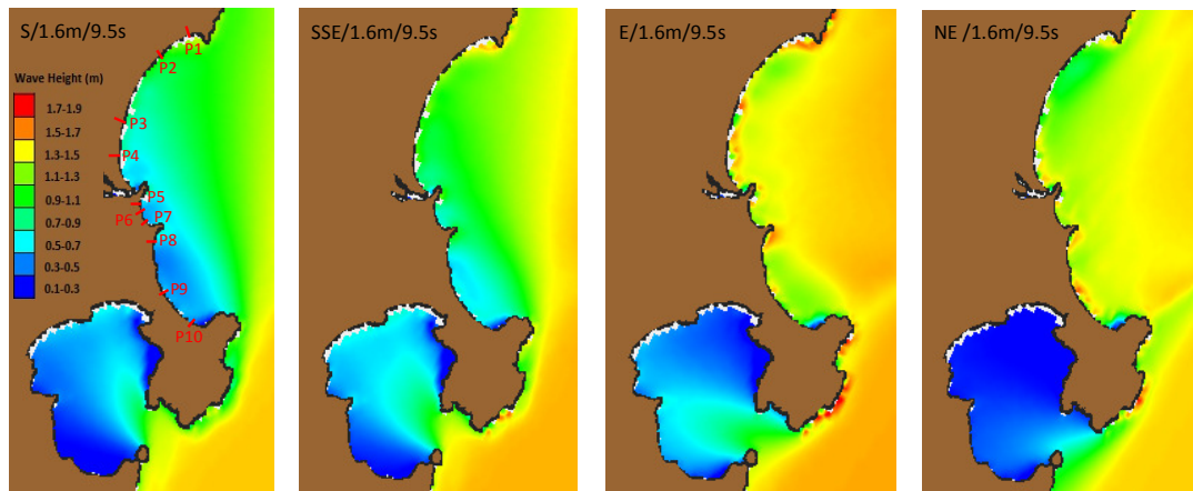
Fig.5: Wave refraction for different direction modelled scenarios. Location of beach profiles is shown on the left.
