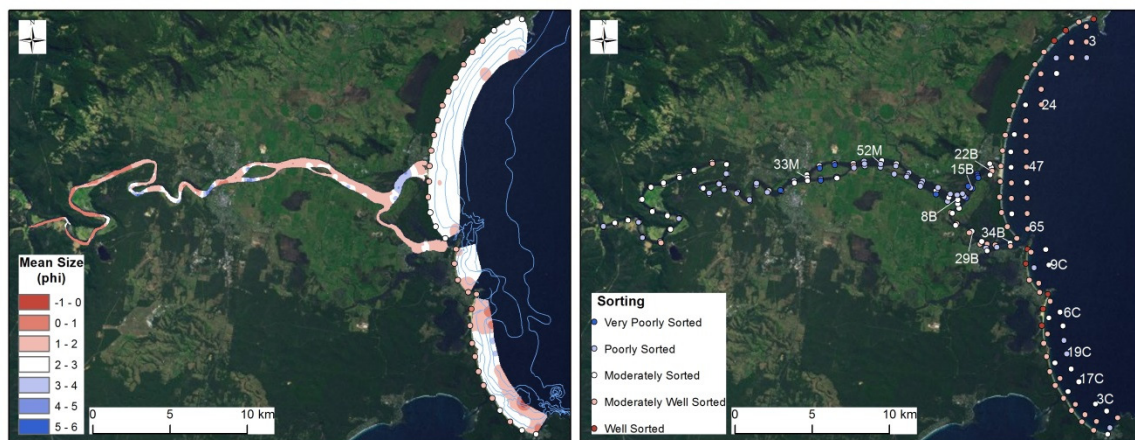
Fig.7: Modern surficial textural distribution of estuarine, beach and offshore sediments in the Shoalhaven coastal compartment. Mean grain size (left) and Sorting degree (right). Samples analyzed for mineralogy are labelled.
