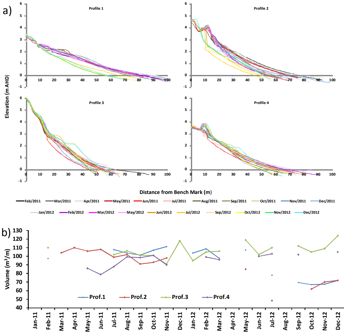
Fig.6: a) Monthly beach profiles using RTK-GPS; b) Monthly beach profile volume change above 0m AHD.
