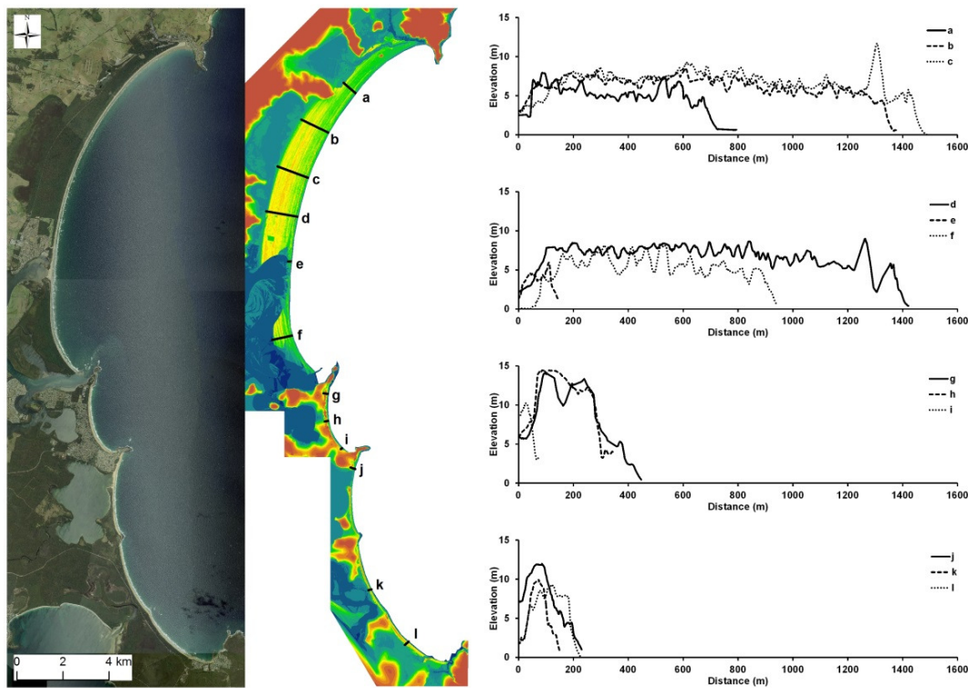
Fig.2: Air photography of the Shoalhaven Coastal Compartment (left), LiDAR data (middle) and cross-sections showing different morphologic types of barriers (right).
