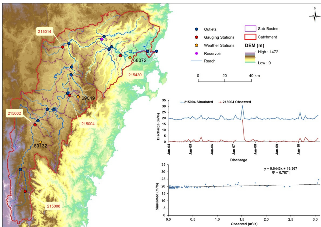
Fig.4: SWAT model monthly simulation during 2004-2010. Simulated x Observed discharge results for Gauging Station 215004 is graphed.
