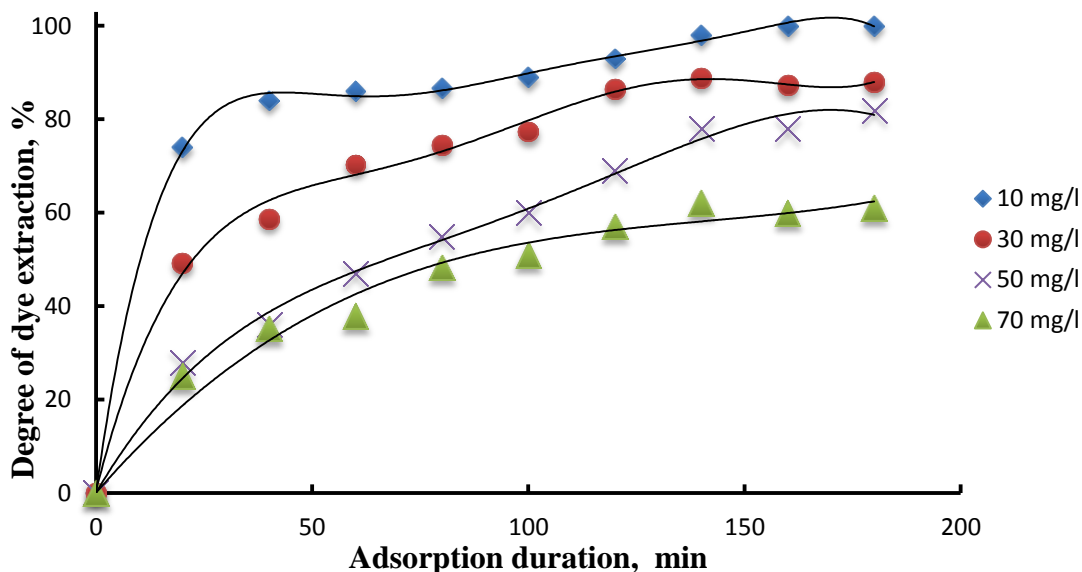
Figure 6. Effect of adsorption duration on the degree of extraction dye
