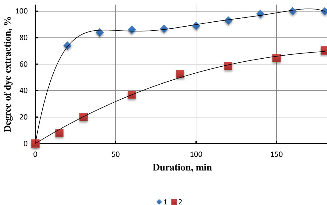
1 – synthesized sorbent; 2 – activated carbon F300 Figure 5. Effect of adsorption duration on the degree of extraction dye
