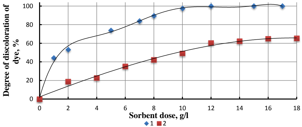
1 – synthesized sorbent; 2 – activated carbon F300 Figure 3. Effect of dose sorbents on removal efficiency of dye
