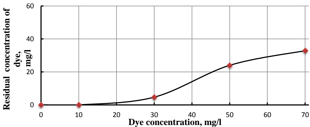
Figure 4. Effect of initial dye concentration "Active brilliant blue KX " on the residual content of dye by synthesized sorbent in water purification
