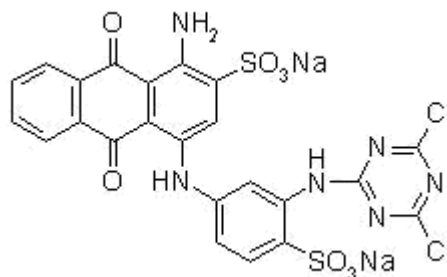
Figure 1 – The structural formula of dye “Active brilliant blue KX”
